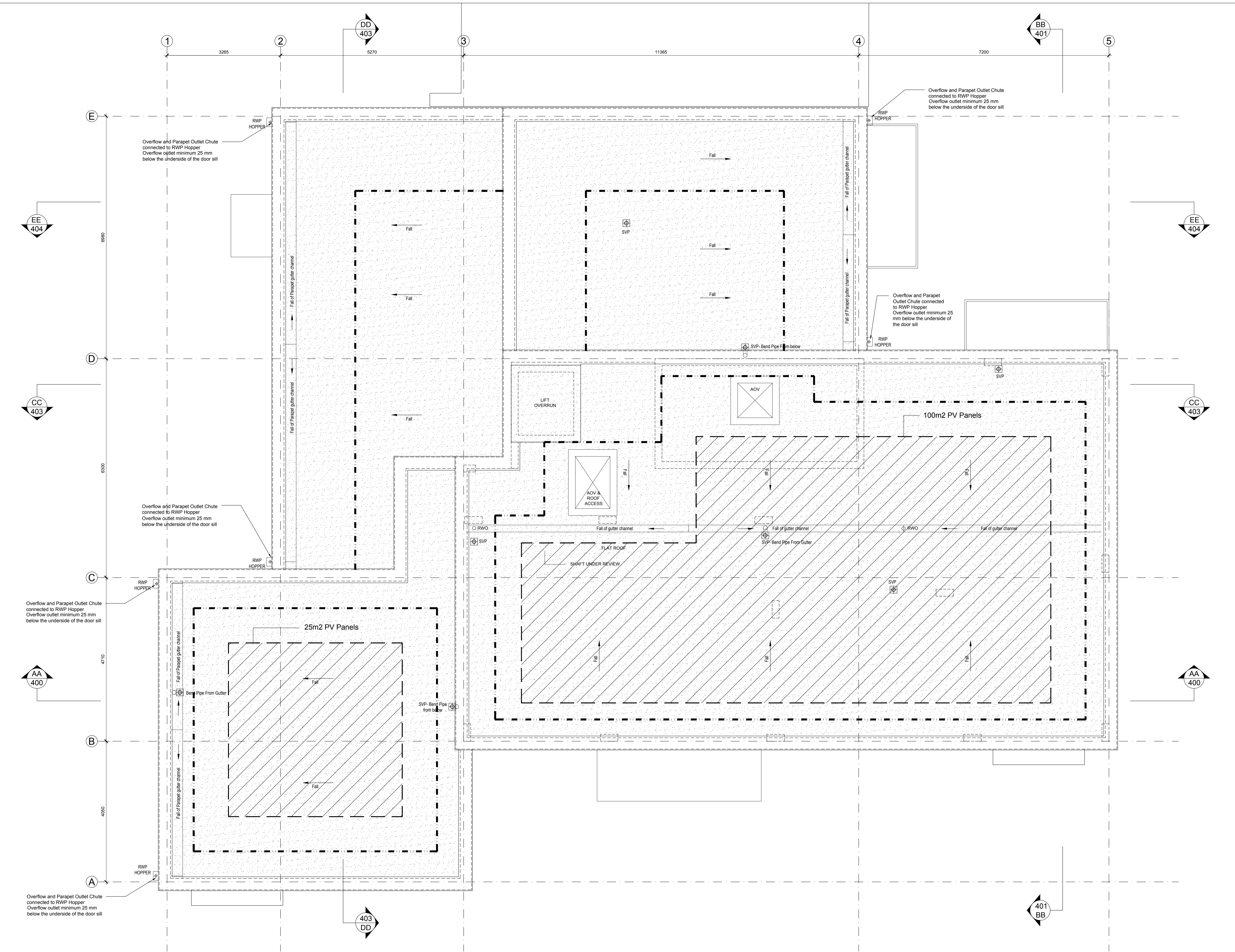
Proposed Roof Plan Scale 1:50
