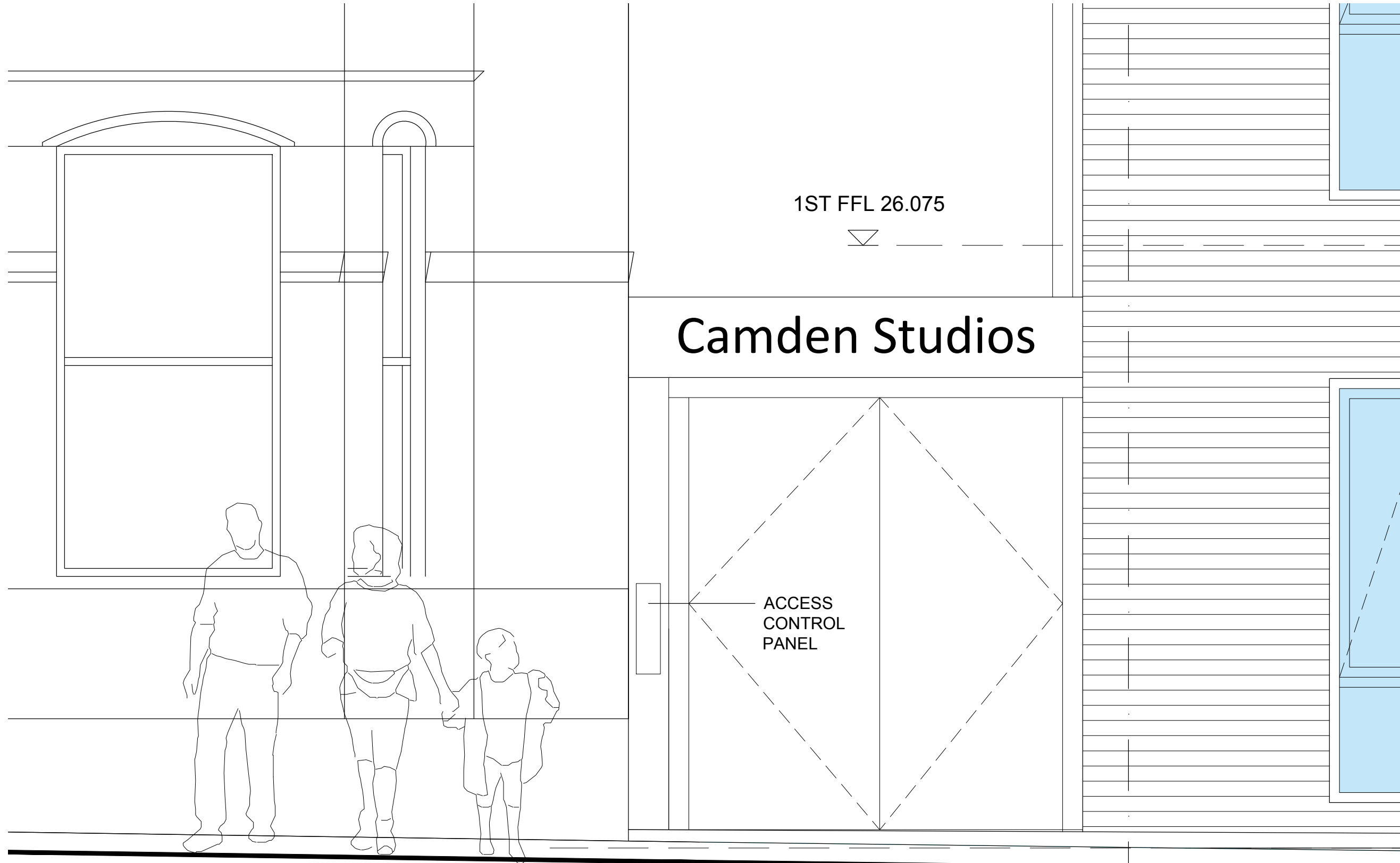
Elevation of Camden Studios Entrance Scale 1:20
