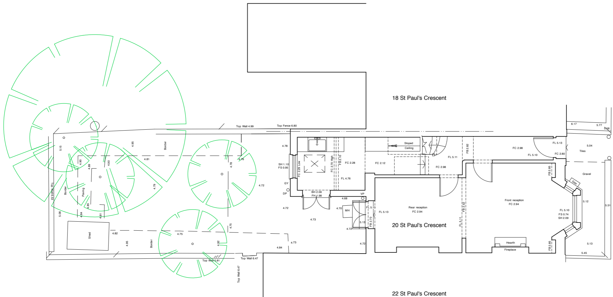
EXISTING SITE PLAN SCALE 1:100@A3
