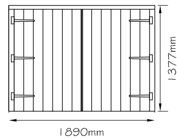
Front Elevation @ 1:50
