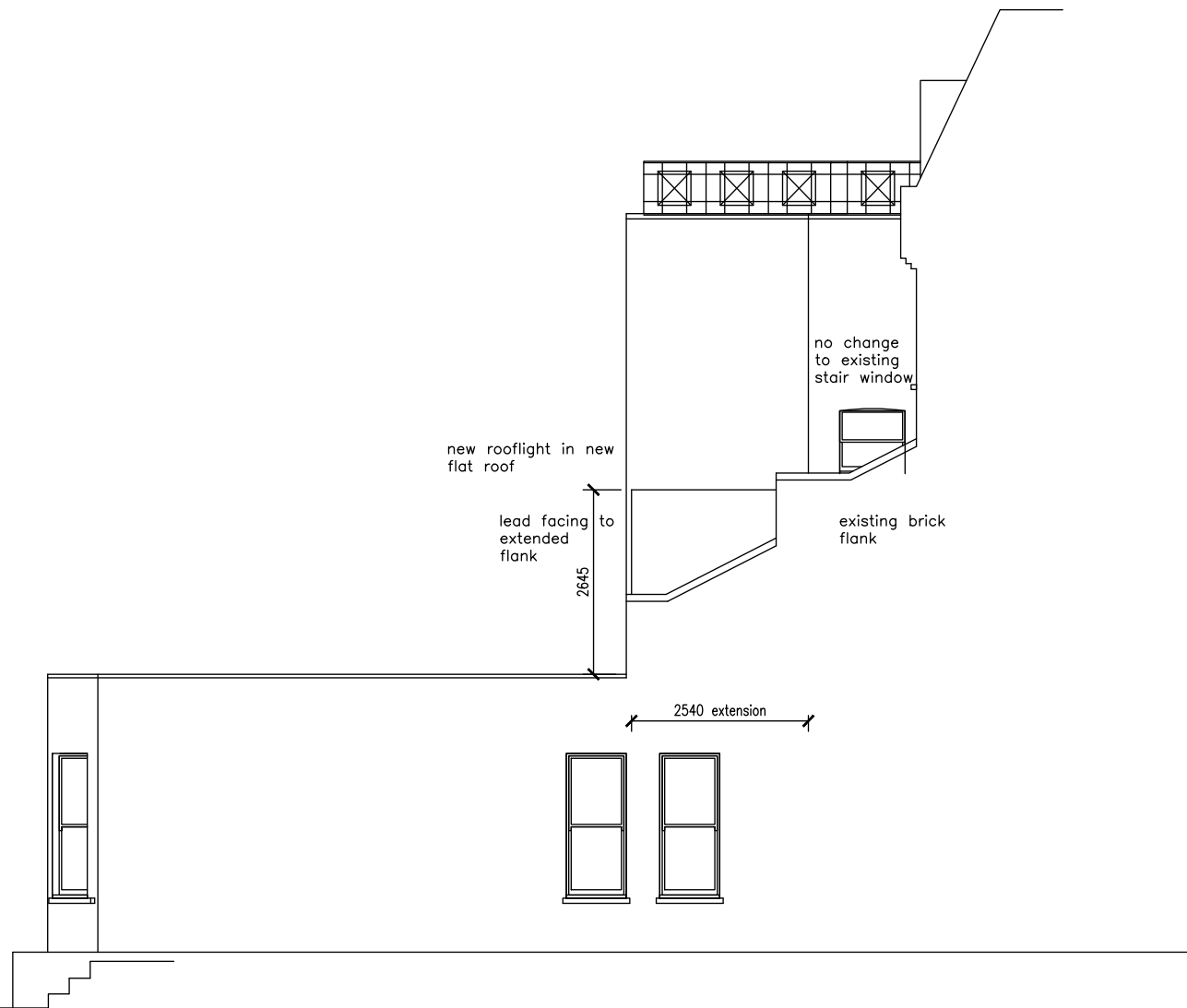
PROPOSED PART SIDE FLANK ELEVATION
