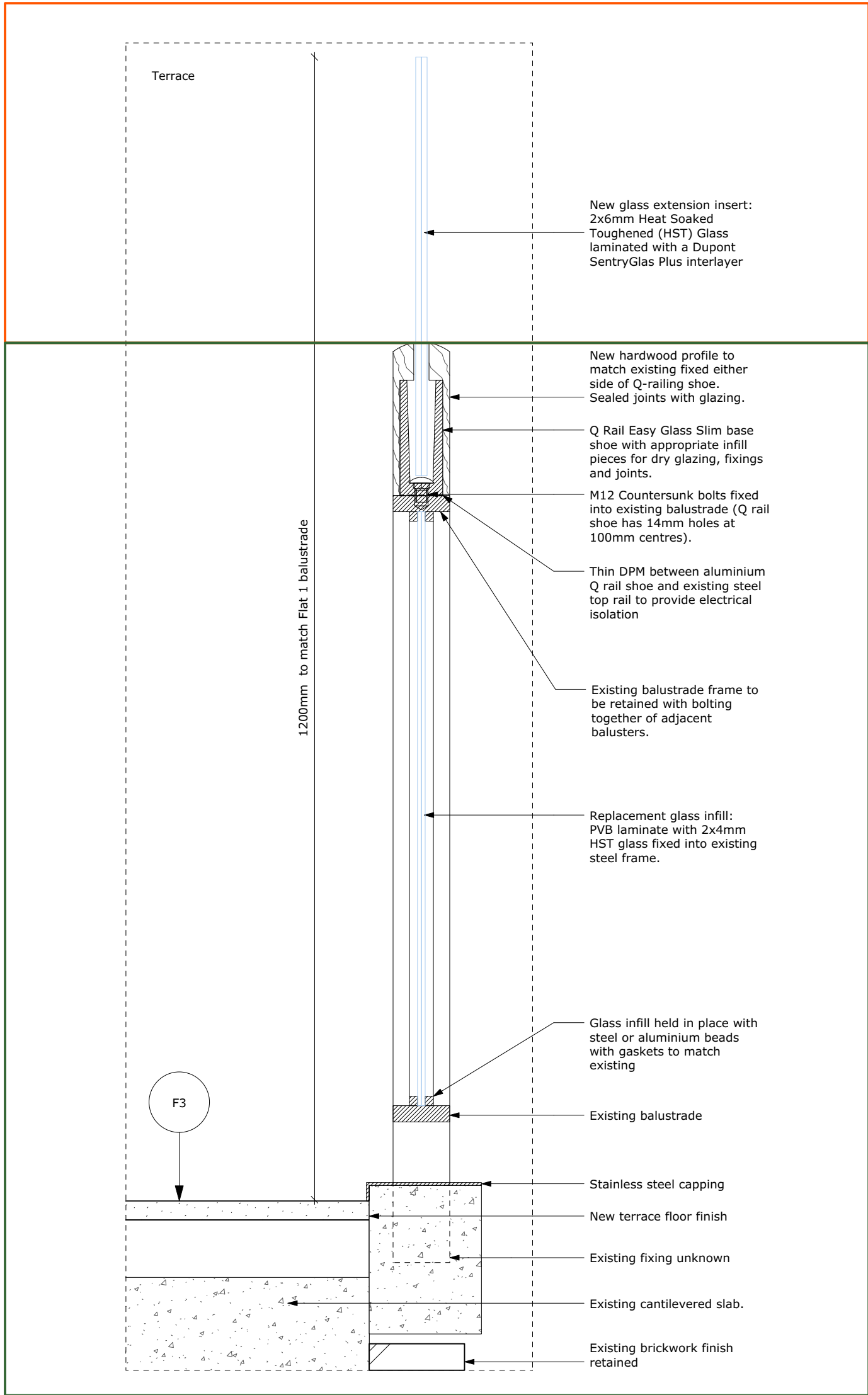
5 Balustrade detail 1:5
