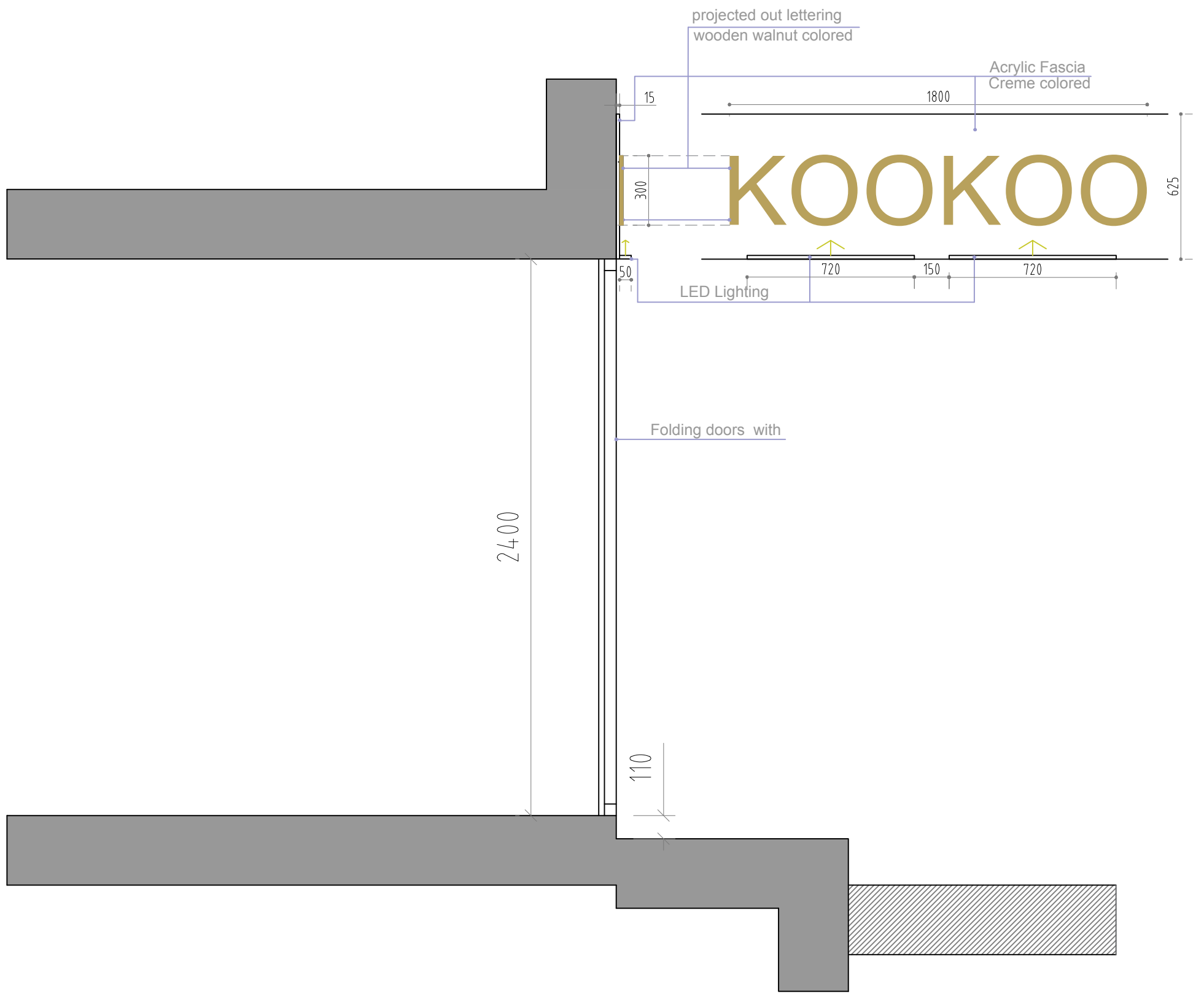
Section B
