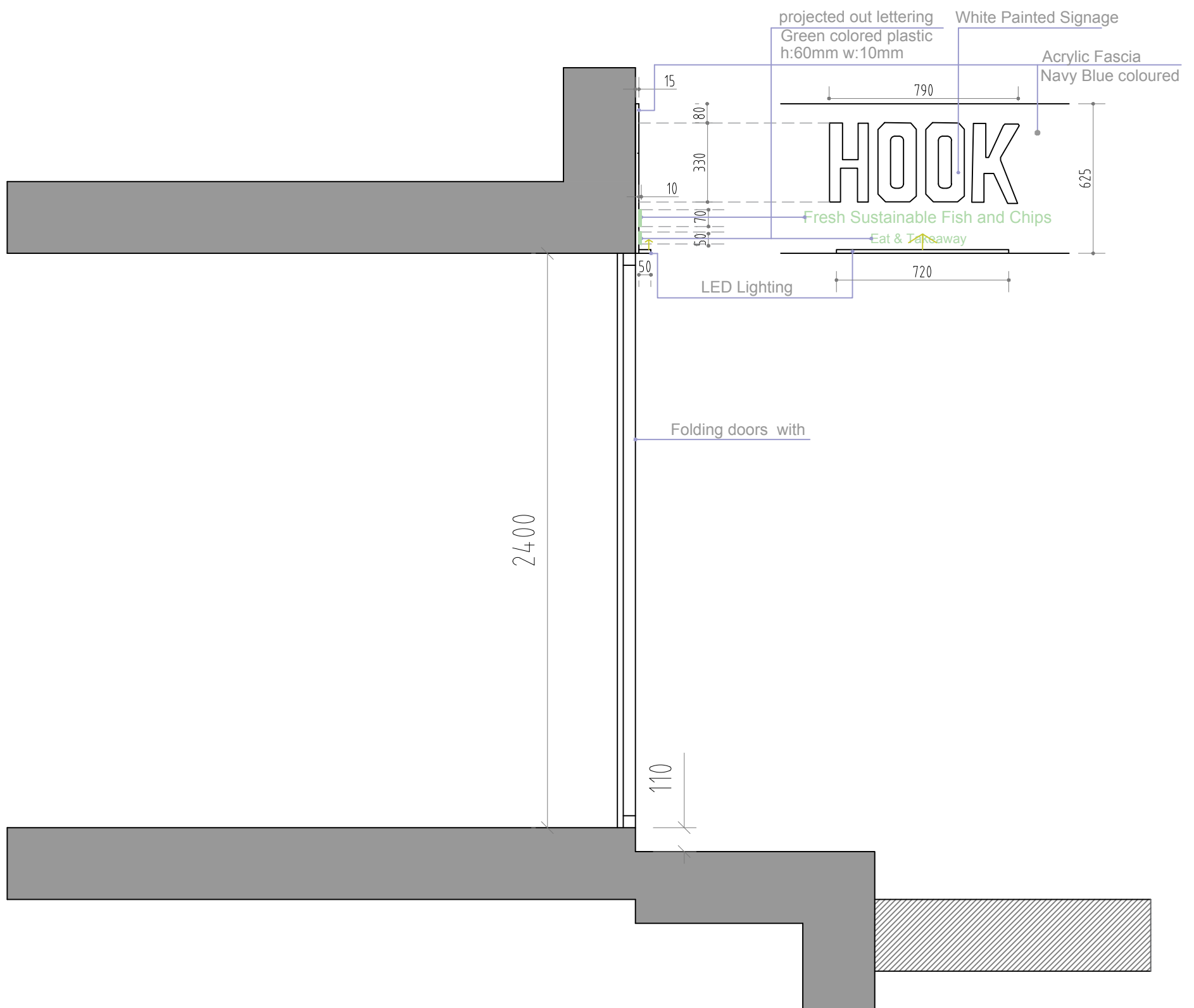
Section A
