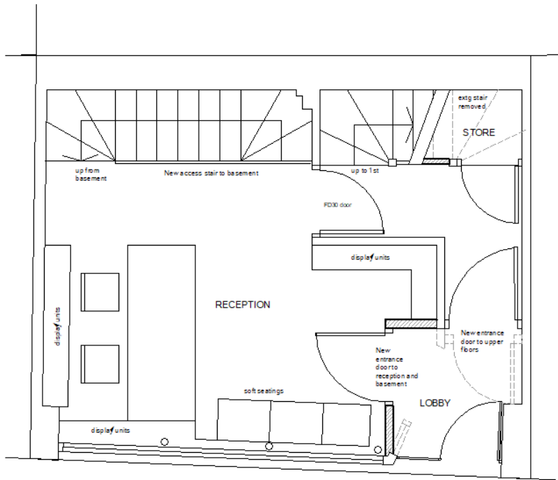
EXISTING GROUND FLOOR PLAN Scale: 1 - 50
