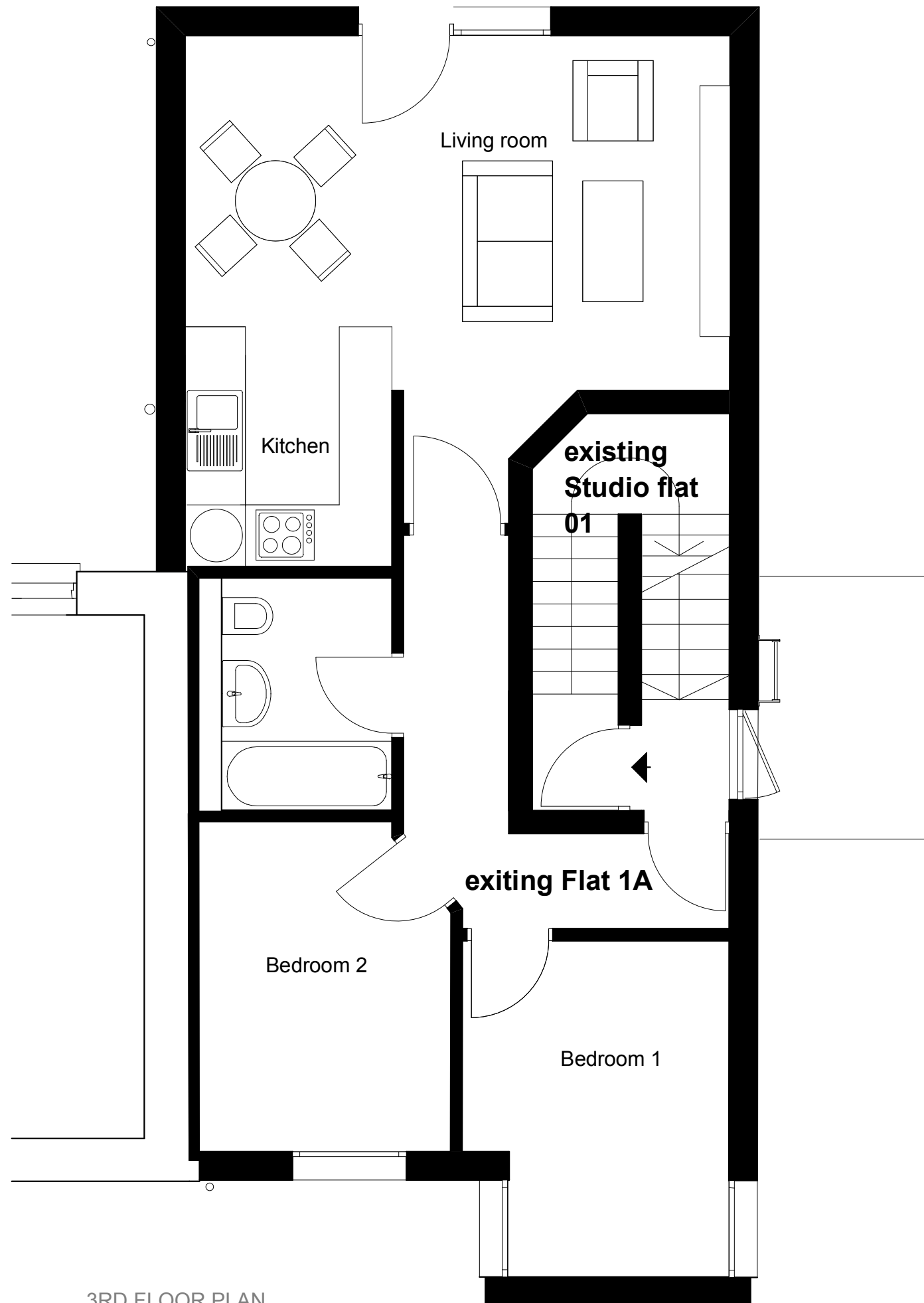
3RD FLOOR PLAN
