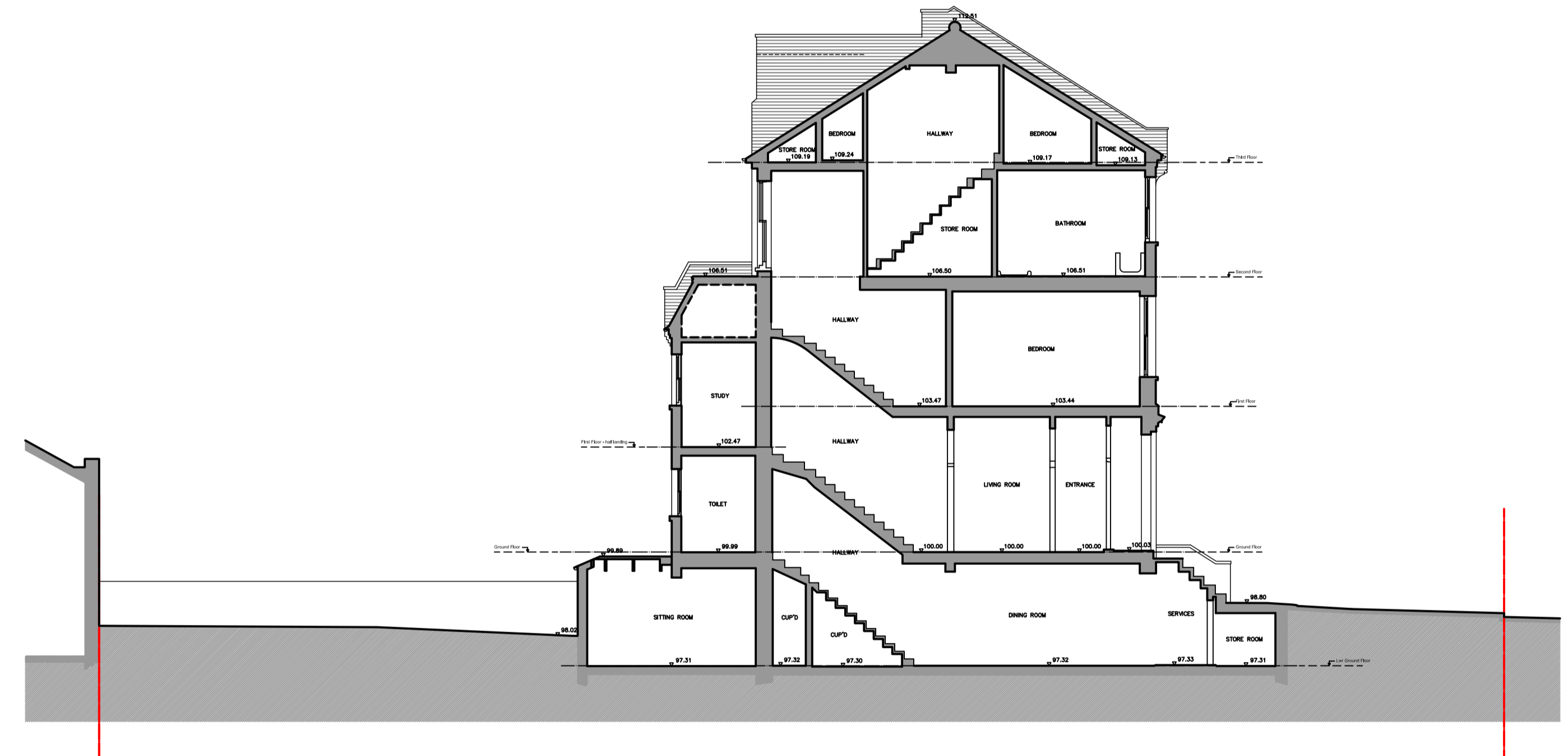
Section B-B
