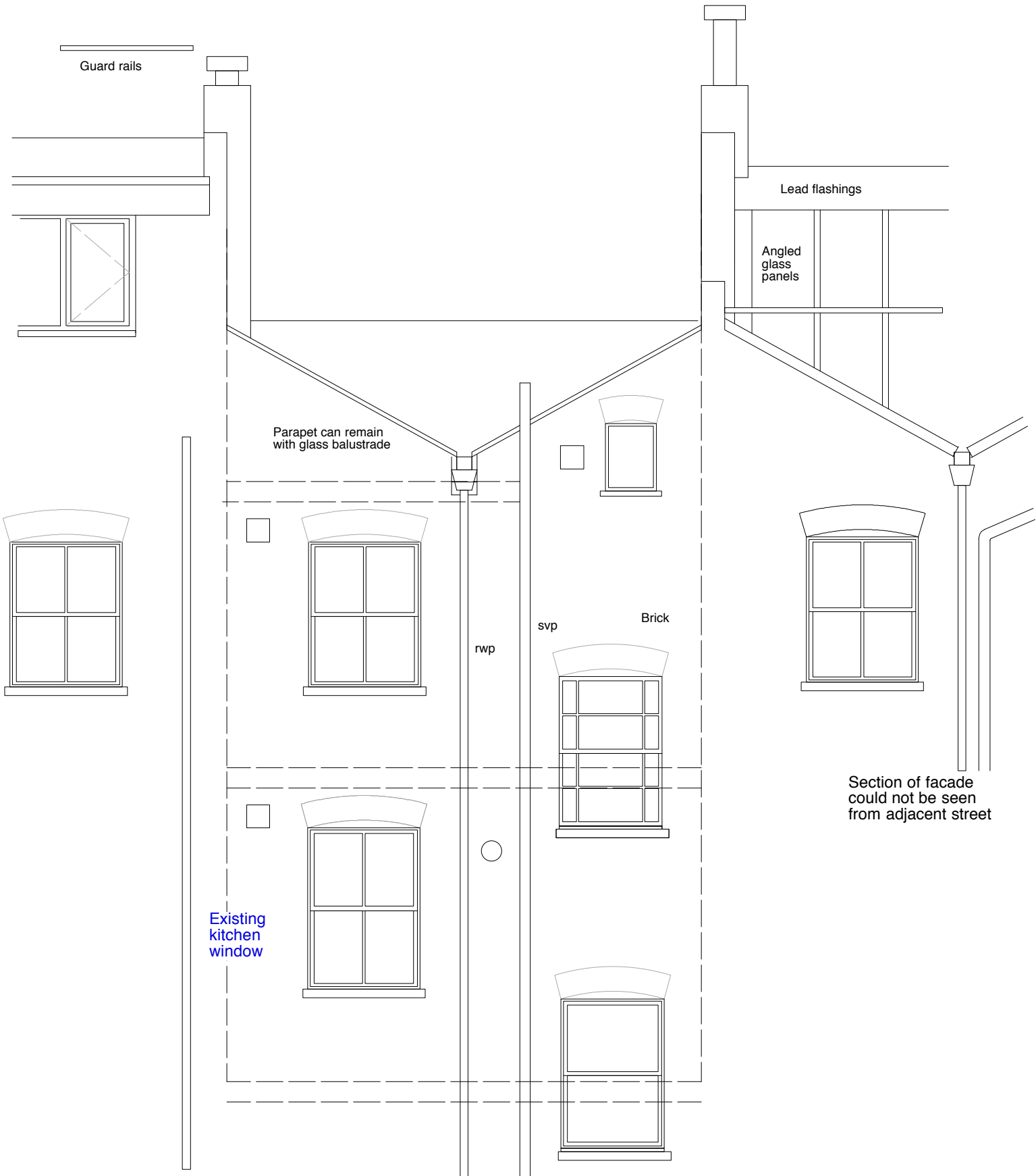
Rear West Elevation
