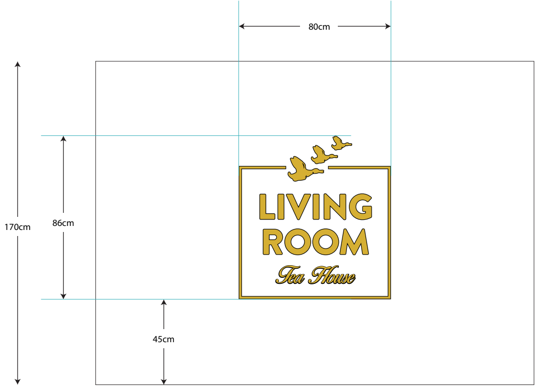
E - Window (Bonny Street elevation)
