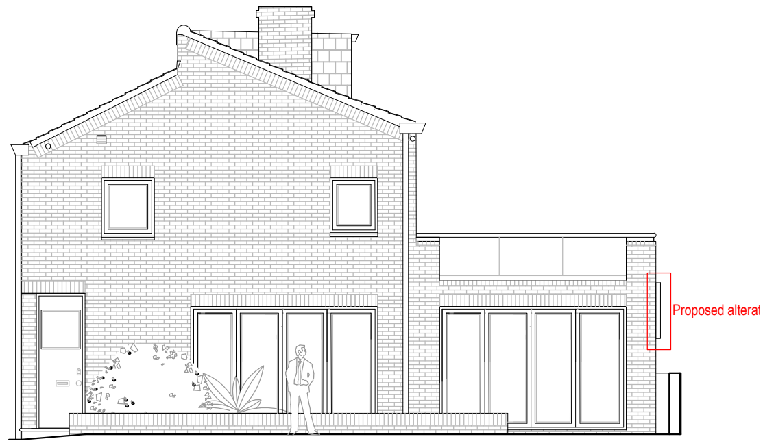
SOUTH-EAST ELEVATION
