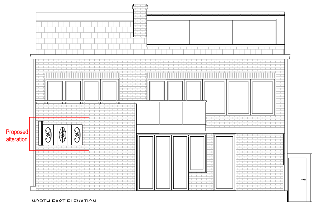
NORTH-EAST ELEVATION
