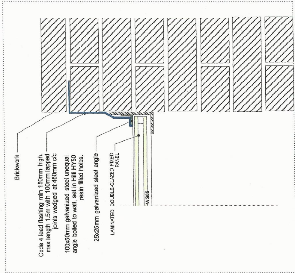
DETAIL-Glass pod /D03 Cross section - SCALE 1:5
