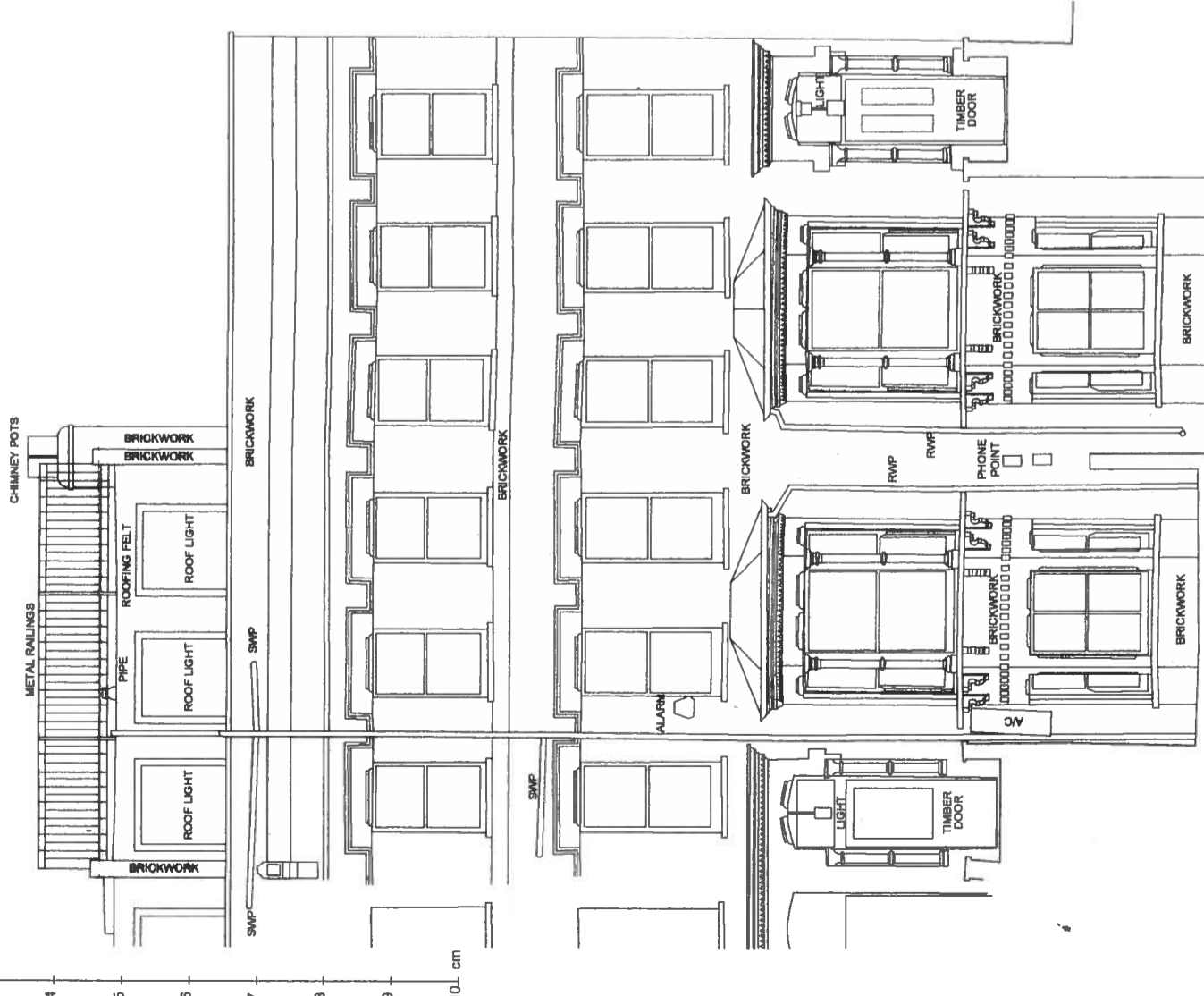
01 EXISTING - FRONT ELEVATION 1:50 @ A1/1, 100@A3
