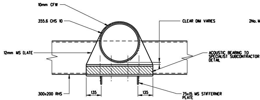
SECTION A 1:10
