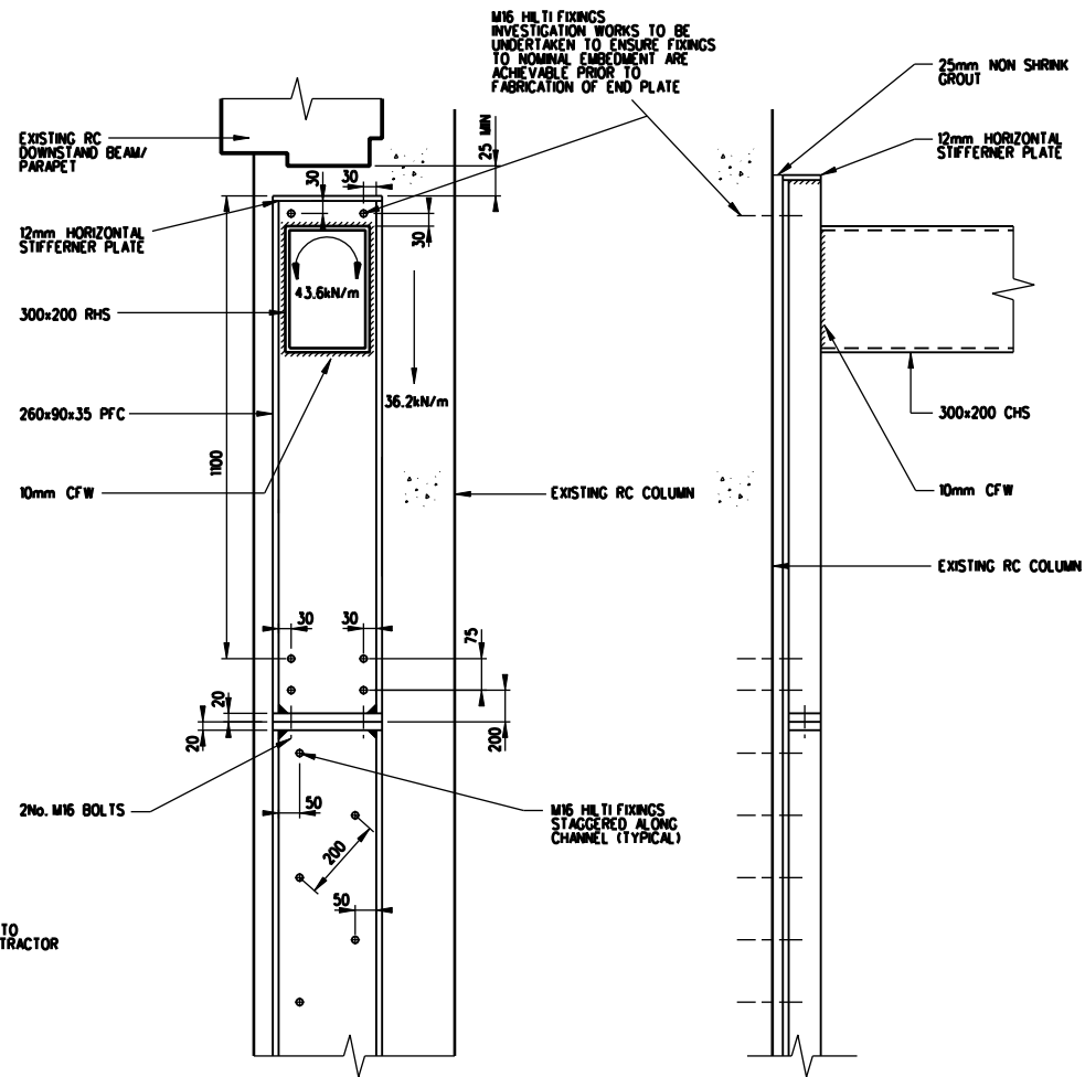
FIXING OF BEAM TO EXISTING RC COLUMN
