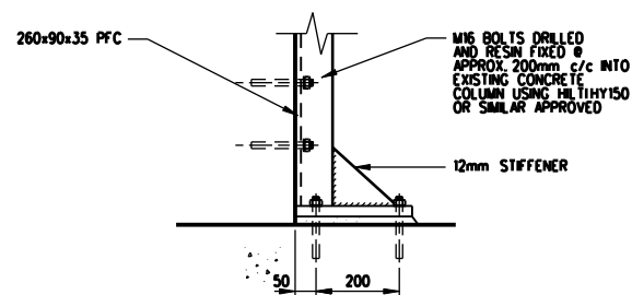
DETAIL 3 1:10
