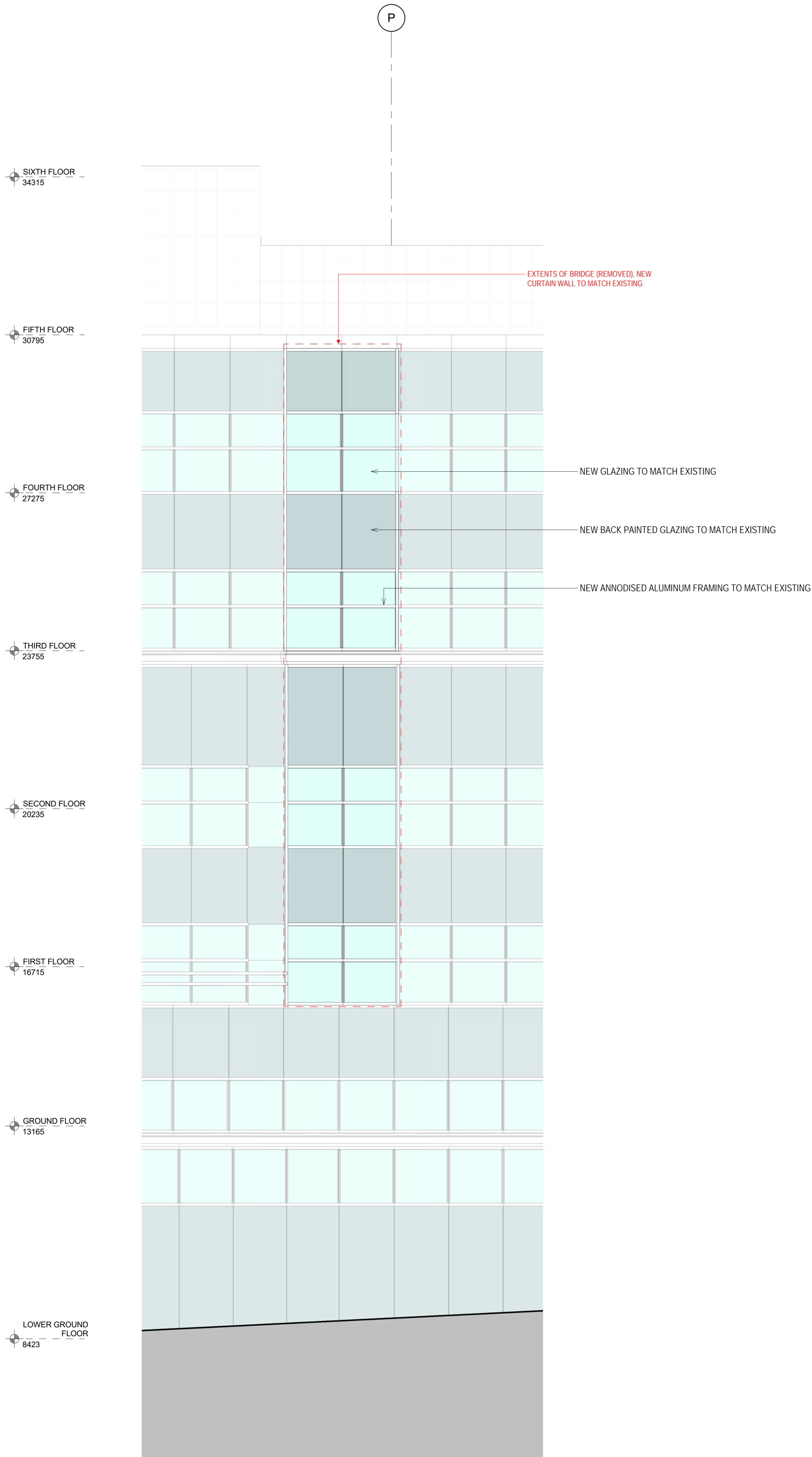
1 SAFFRON HILL ELEVATION BAY STUDY (GRID P) 1:50
