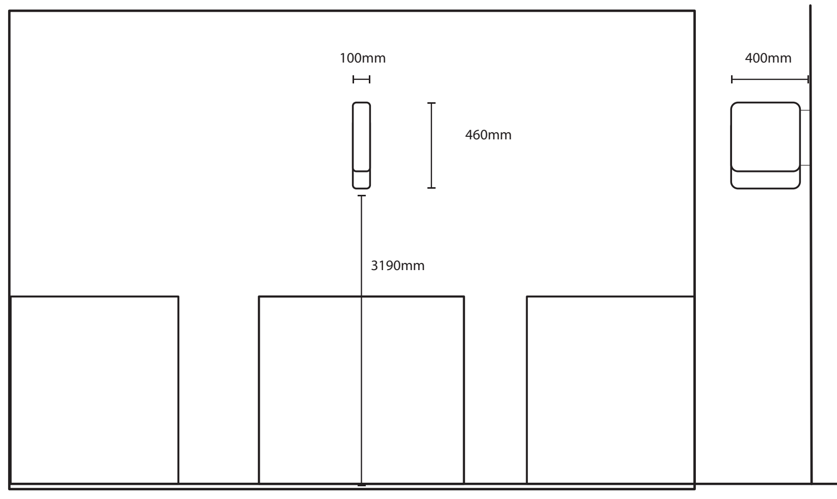
Cheries Mews Front Elevation
