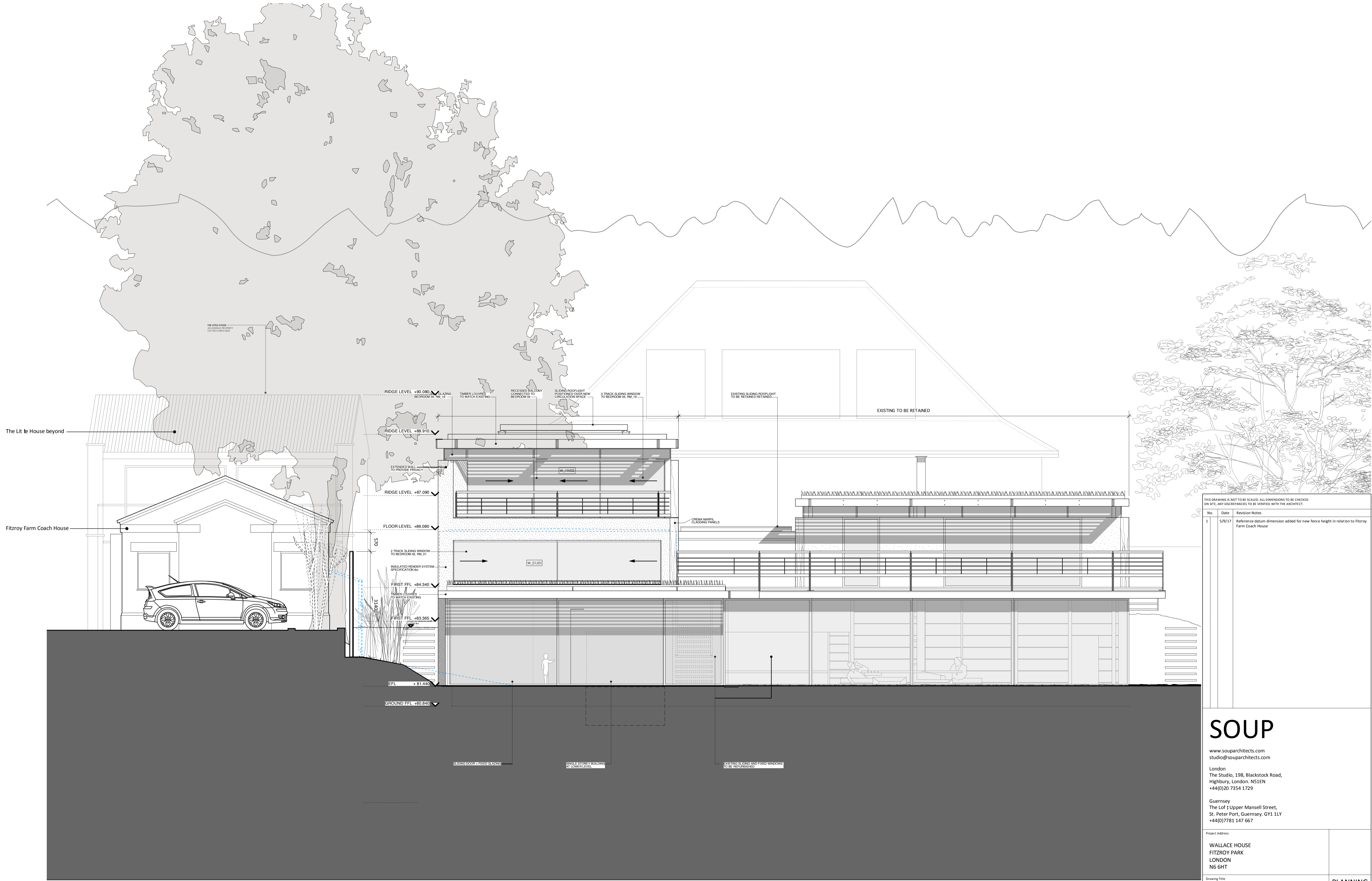
01 PROPOSED SOUTH WEST ELEVATION SCALE: 1:50 @ A1
