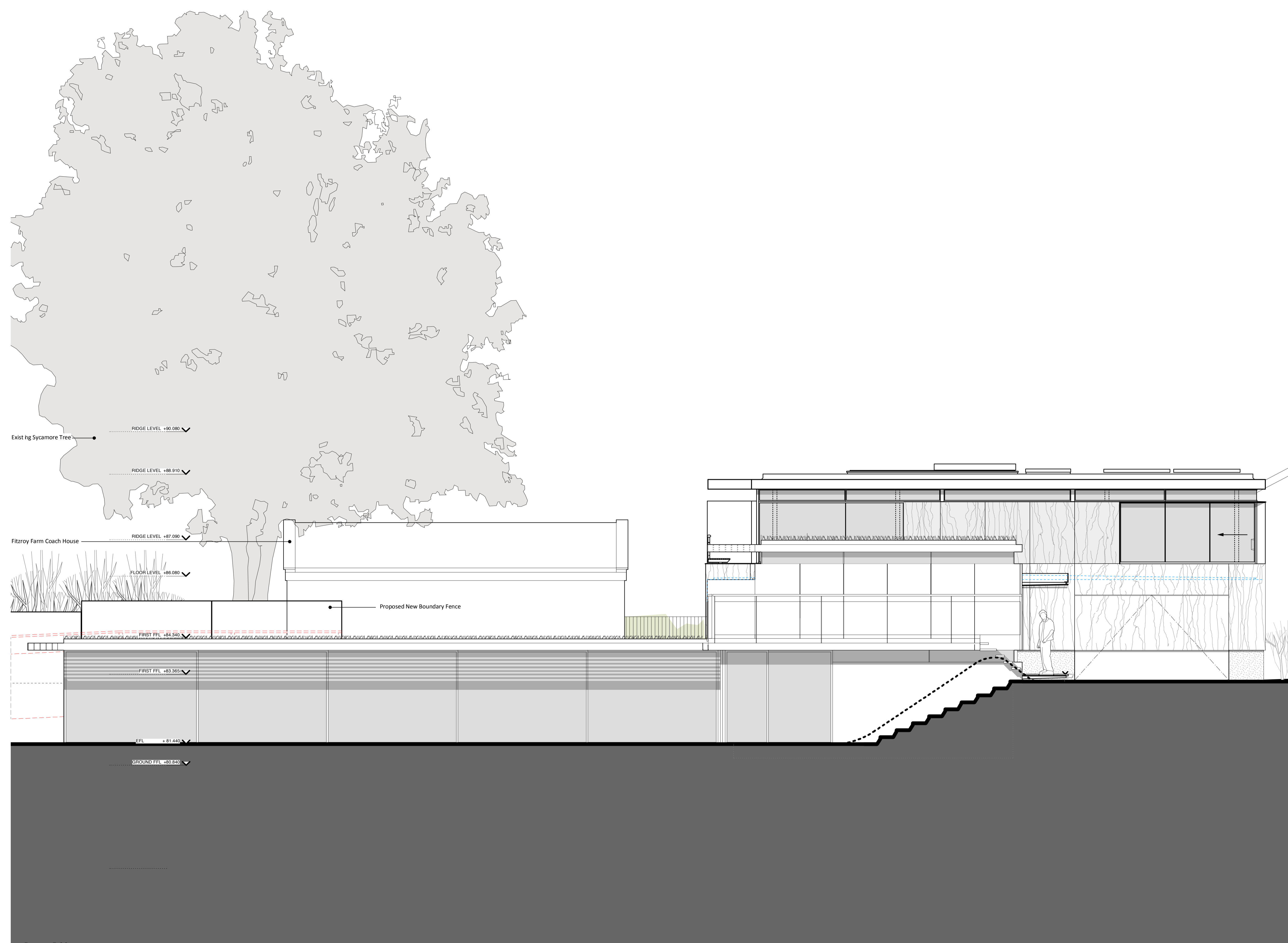
01 PROPOSED SOUTH EAST ELEVATION SCALE: 1:50 @ A1
