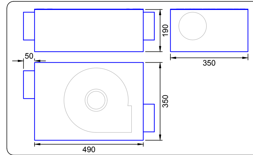
Typical Extract Fan Scale: 1:10
