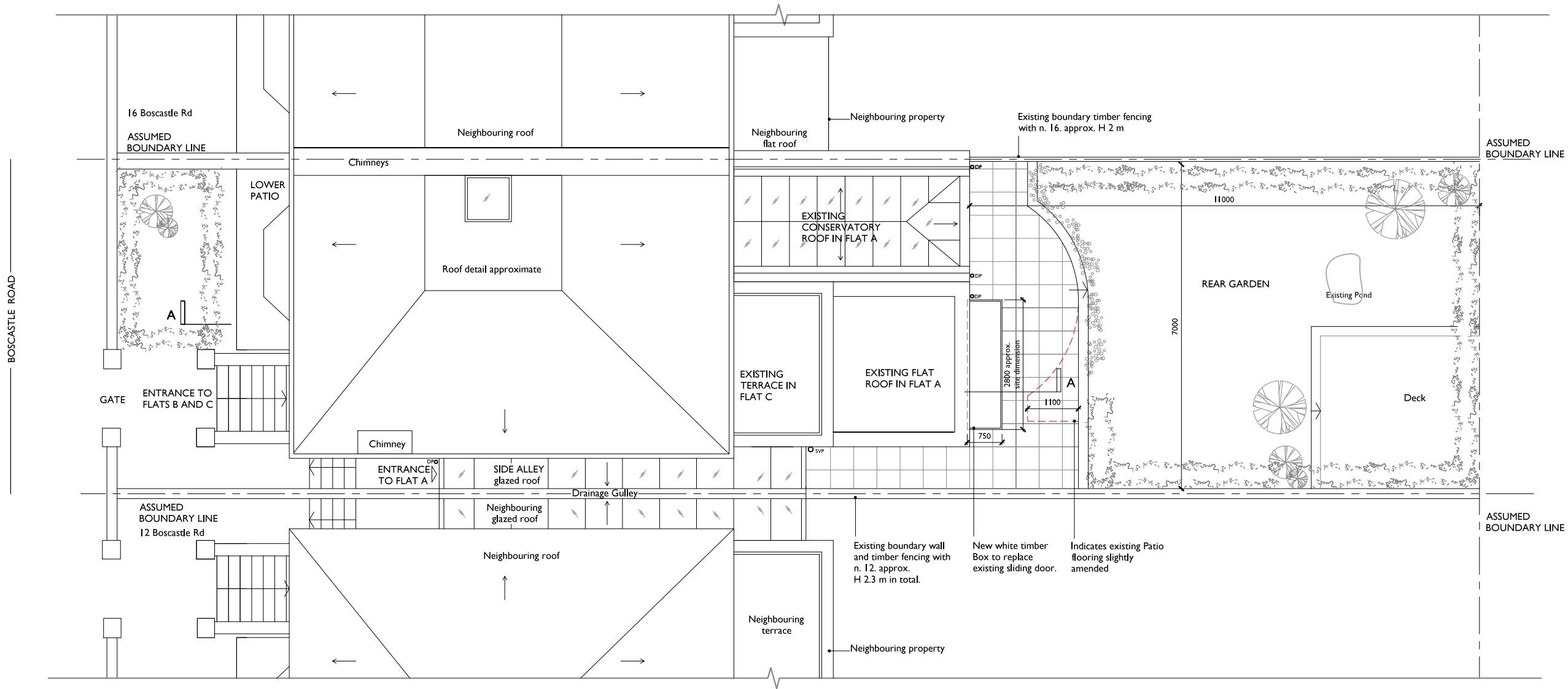
SITE AND ROOF PLAN AS PROPOSED
