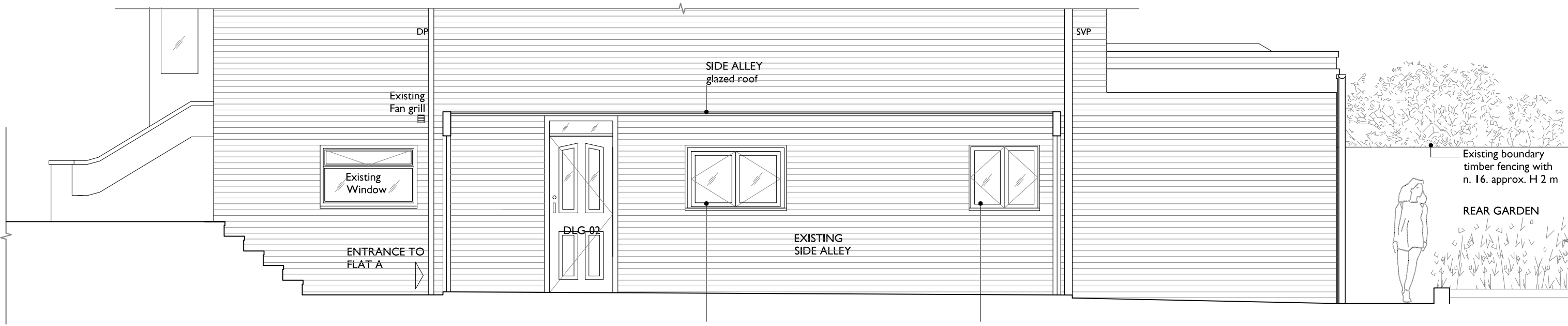
PART SOUTH SIDE ELEVATION AS EXISTING
