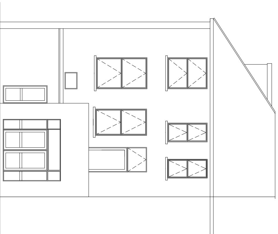
REAR ELEVATION
