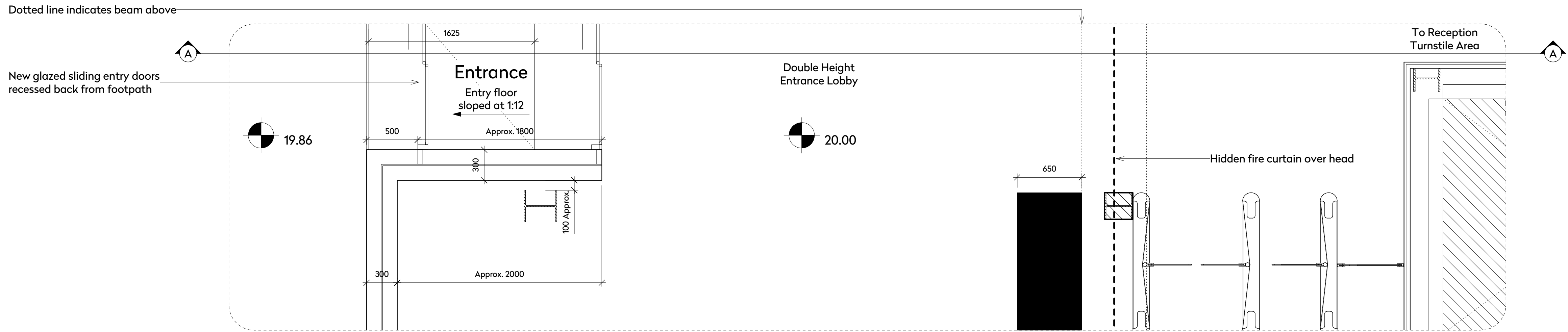
01 New Entry Facade Plan 1:25@A1/1:50@A3
