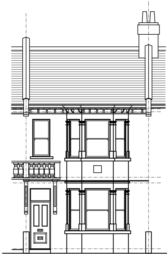
PROPOSED FRONT ELEVATION (no change)
