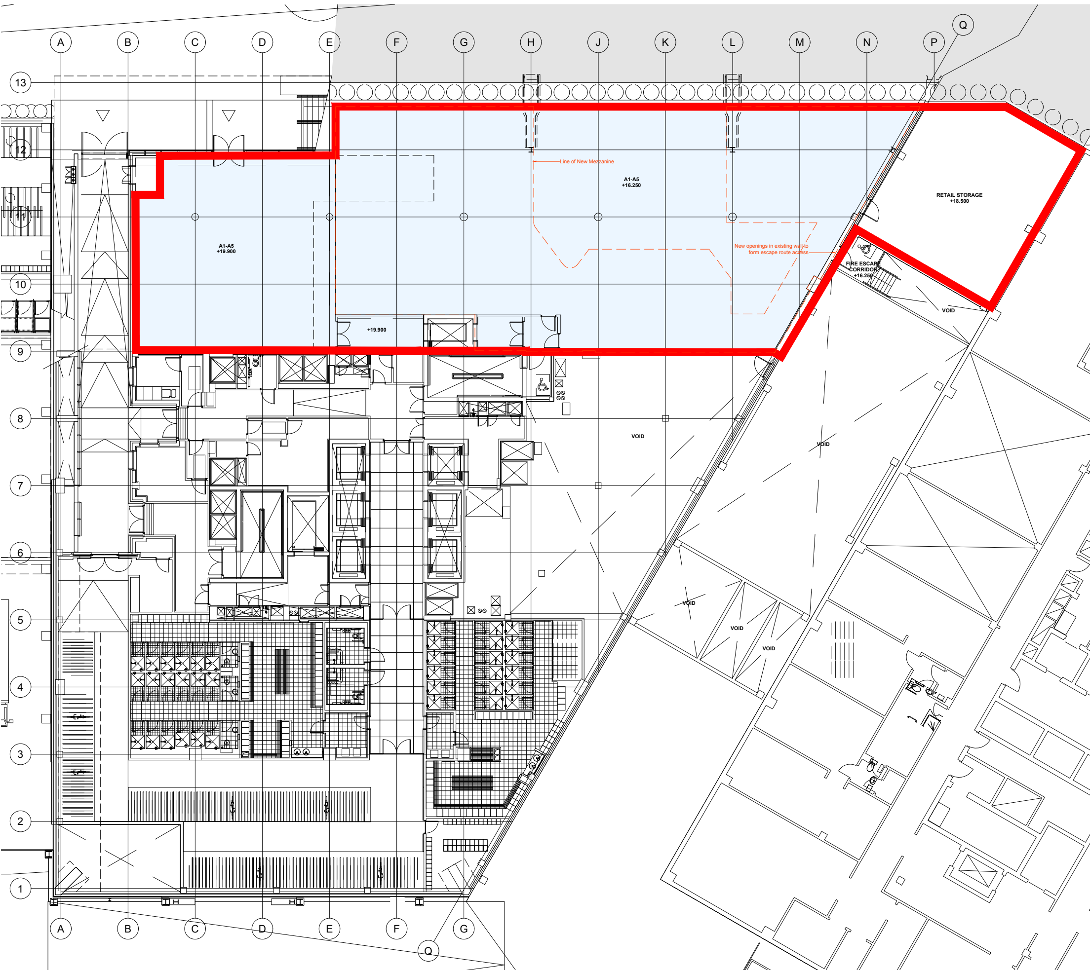
1:250@A3 EXISTING UPPER BASEMENT & LOWER GROUND PLAN
