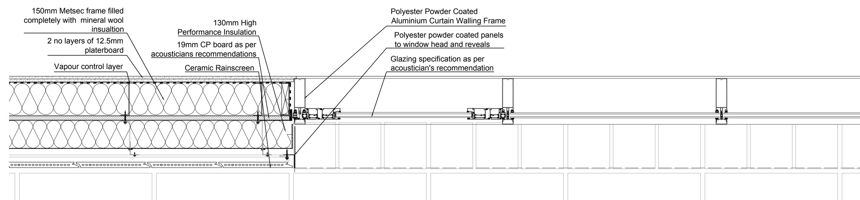
01 CURTAIN WALLING - GROUND Plan 1:10
