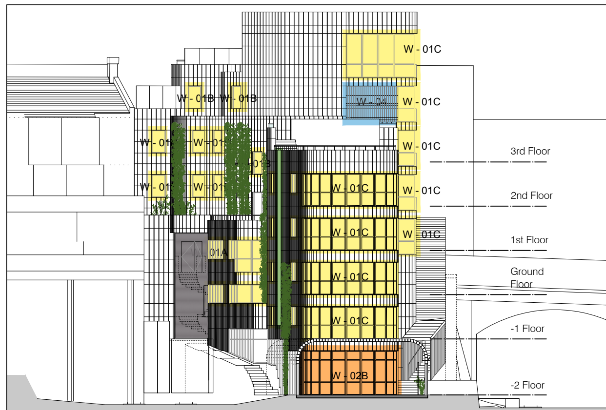
Window Types Elevation 1:250
