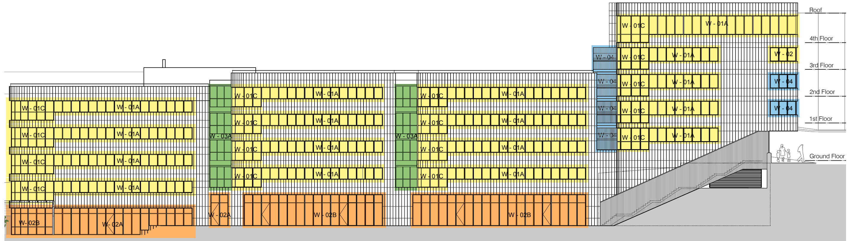
Window Types Elevation 1:250
