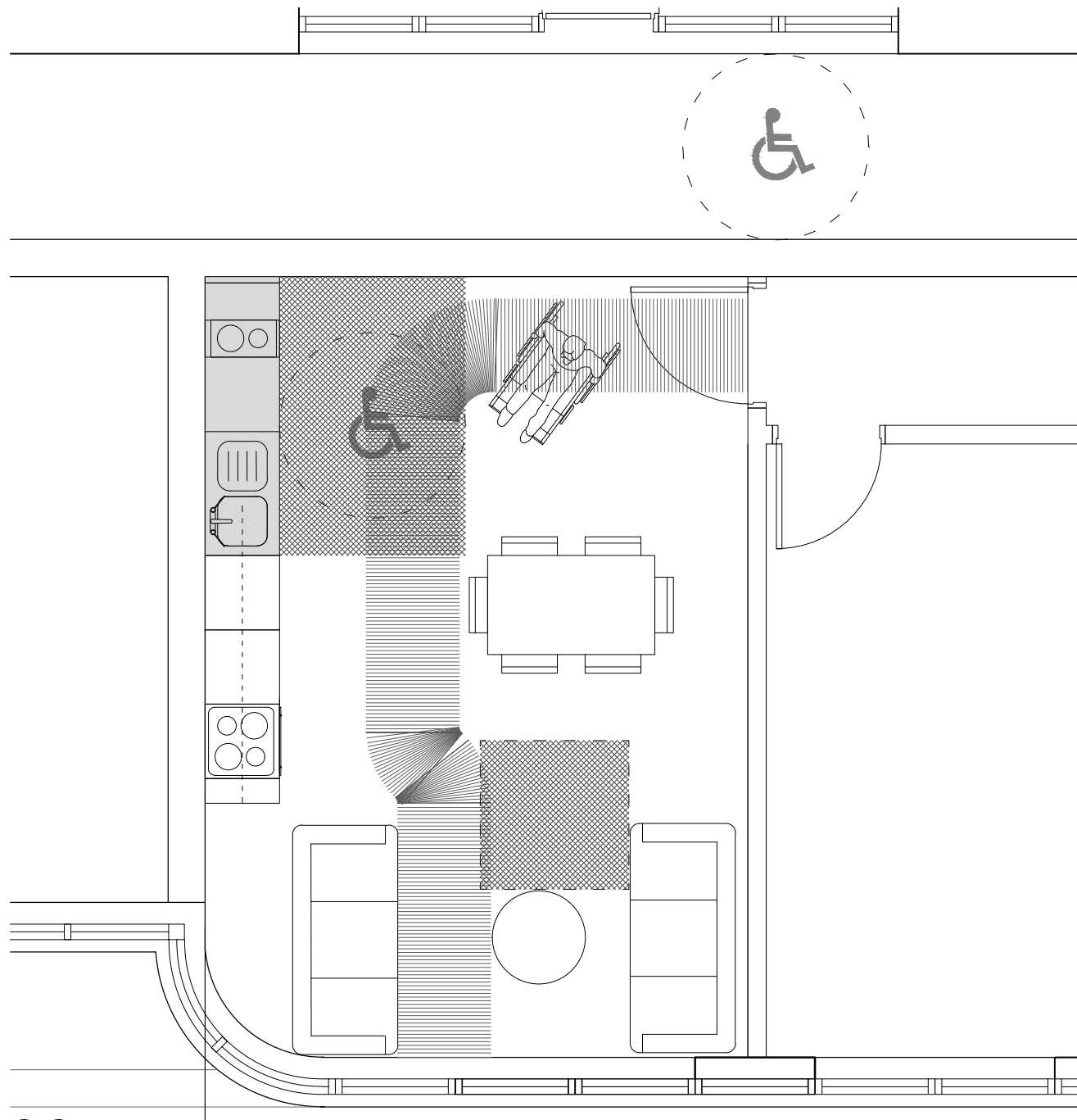
02 Wheelchair Room - Common Room Cluster Plan 1:50
