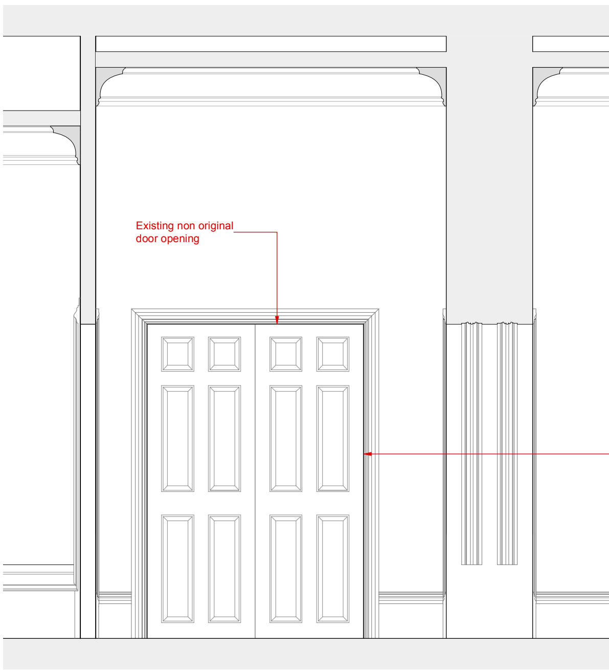
Existing Elevation E @ 1:25
