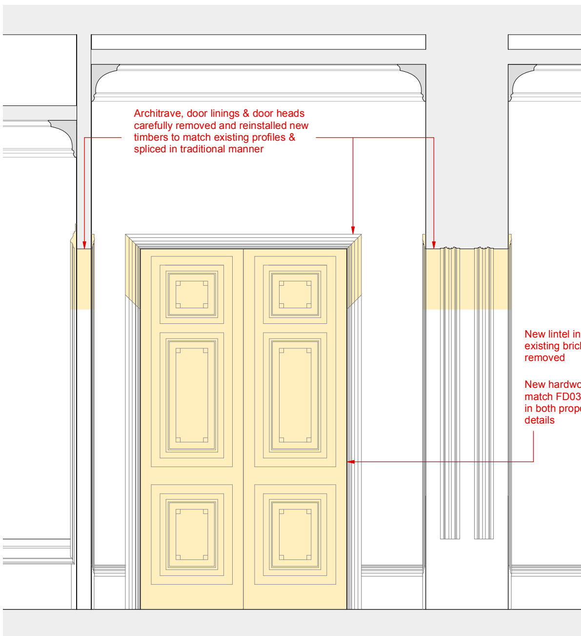
Proposed Elevation E @ 1:25
