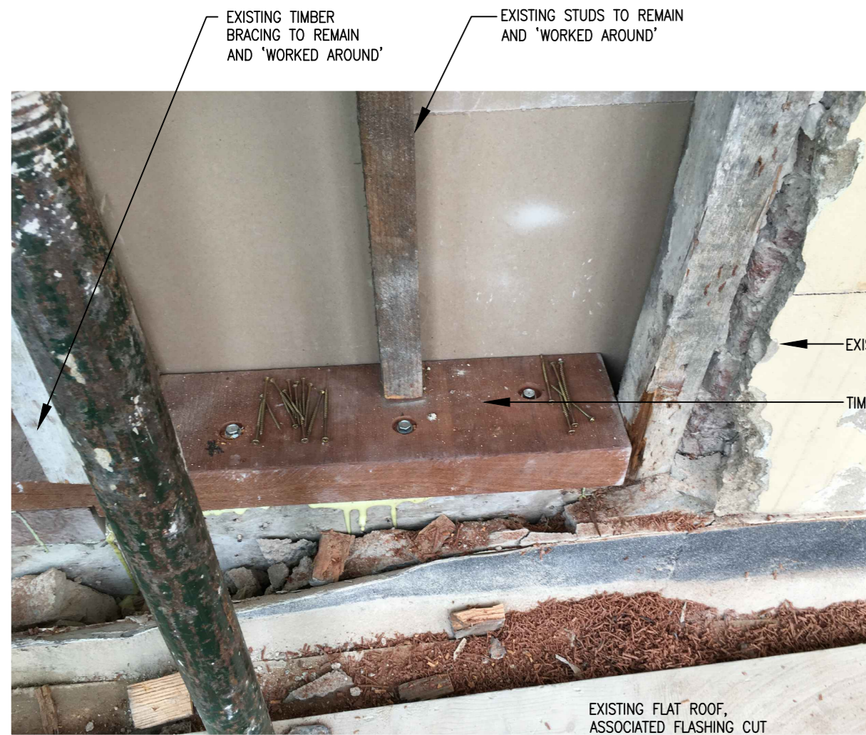
IMAGE OF EXISTING EXTERNAL WALL IN THE PROCESS OF REFURBISHMENT
