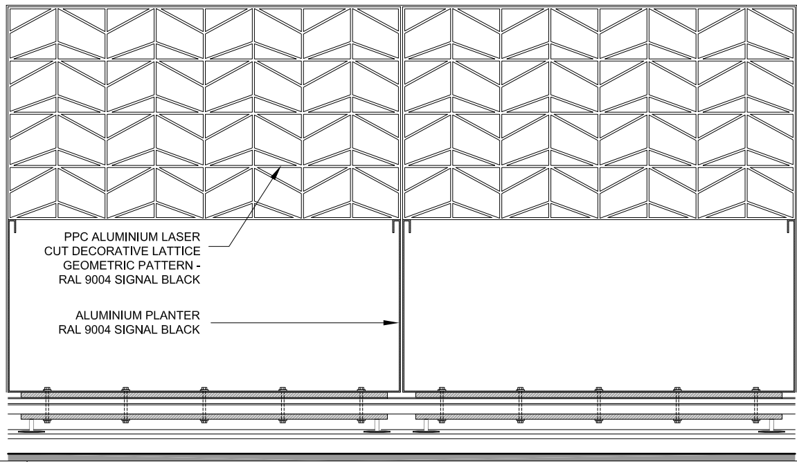
01 PLANTERS - SECTION AA
