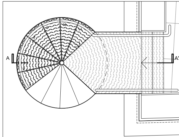
04 SPIRAL STAIR - PLAN
