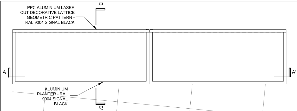
03 PLANTERS - PLAN
