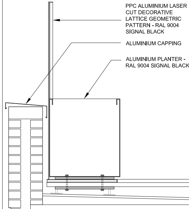
02 PLANTERS - SECTION BB
