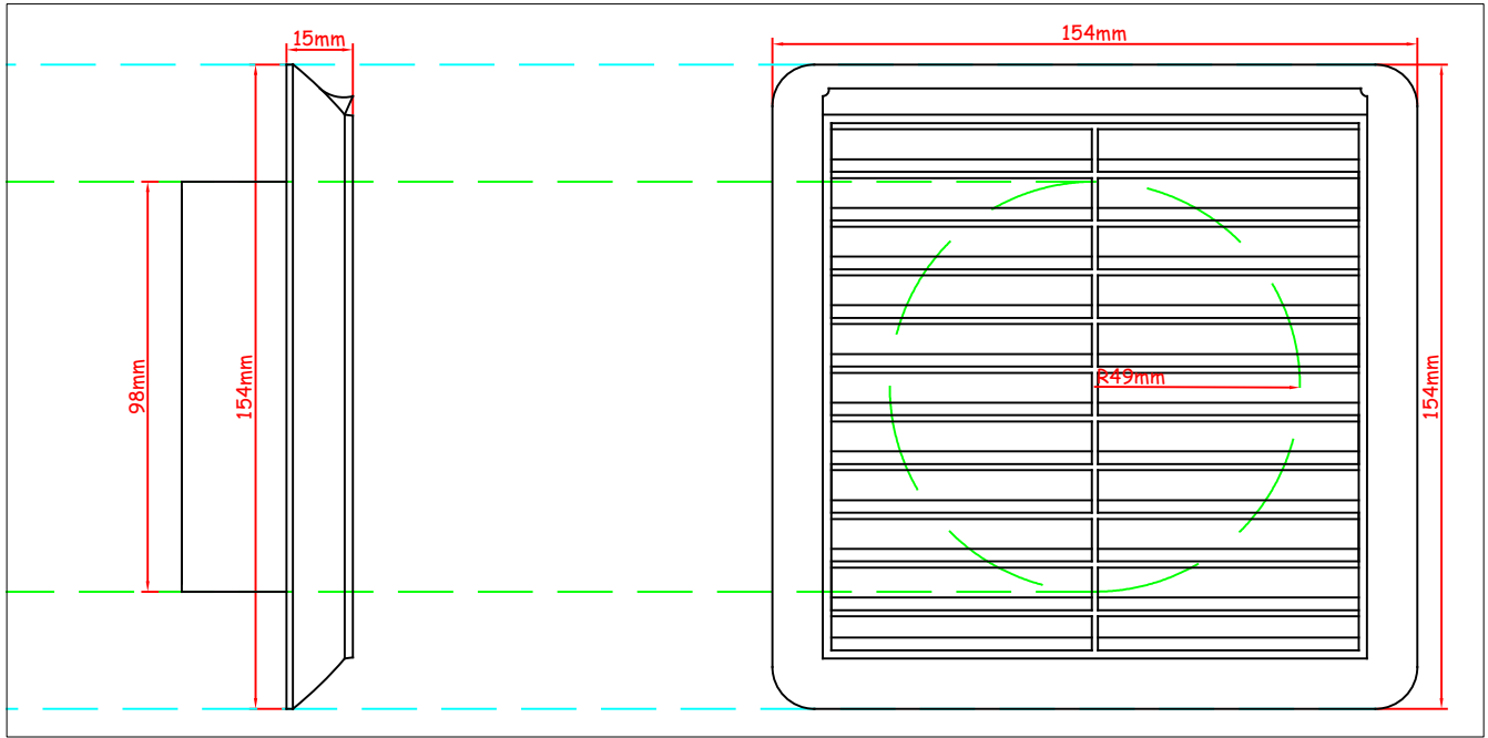
Sonair vent Cowl - Side And Front Elevations. (Scale 1: 2 @ A4)
