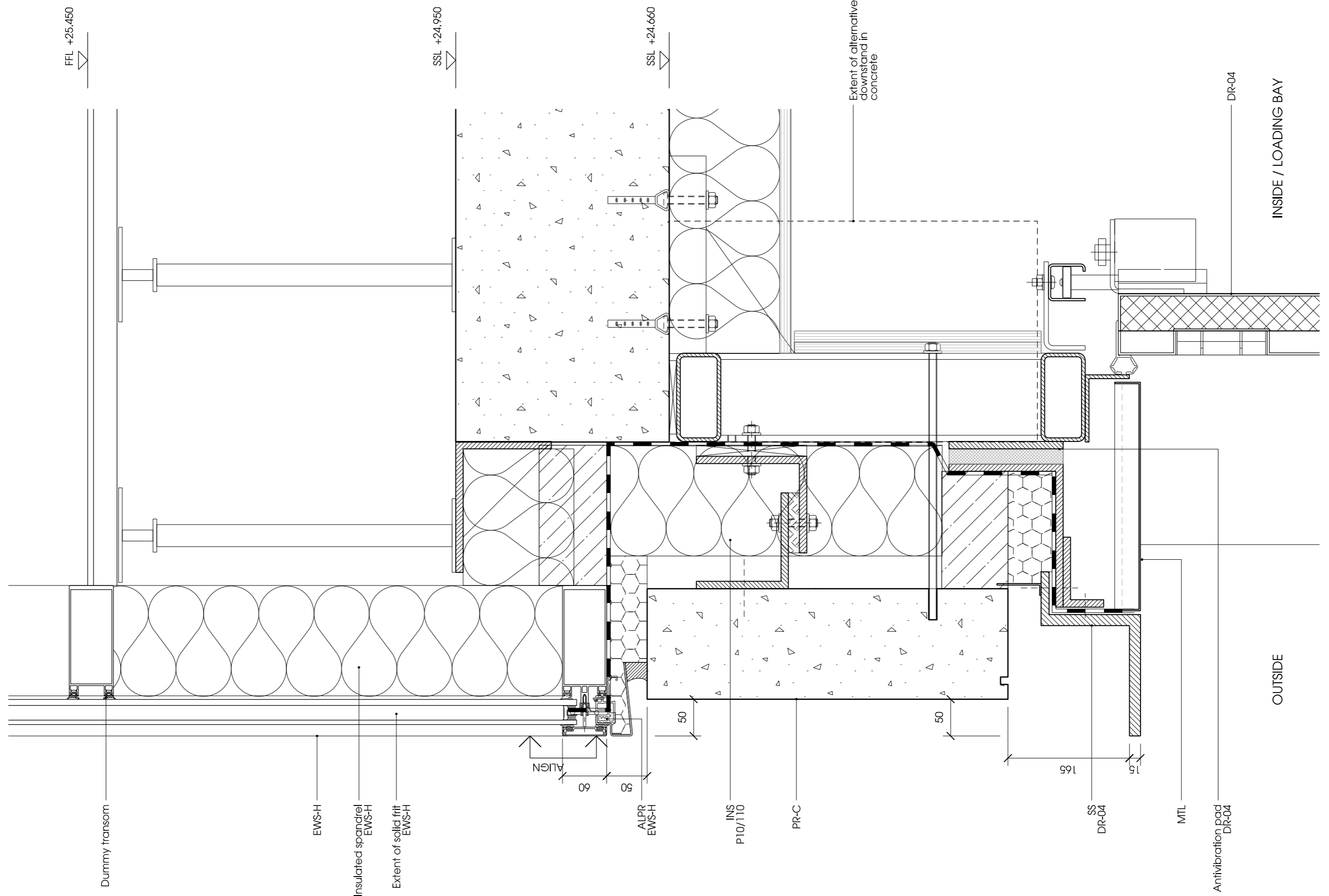
01 Loading bay door head detail 21_563 Refer to drawing 02/21_106
