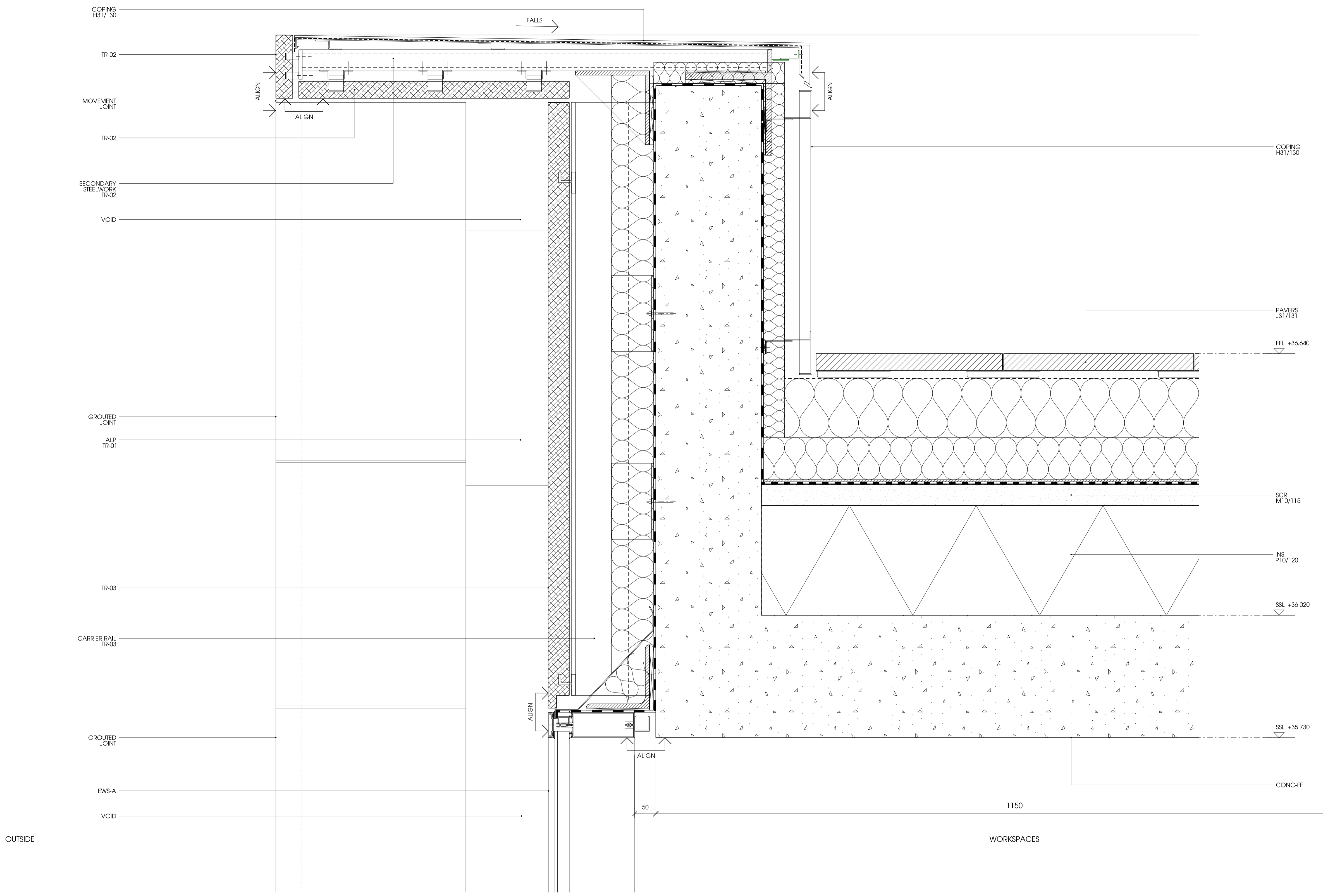
01 Typical Fourth Floor Parapet Detail 21_526 Refer to drawing 21_100
