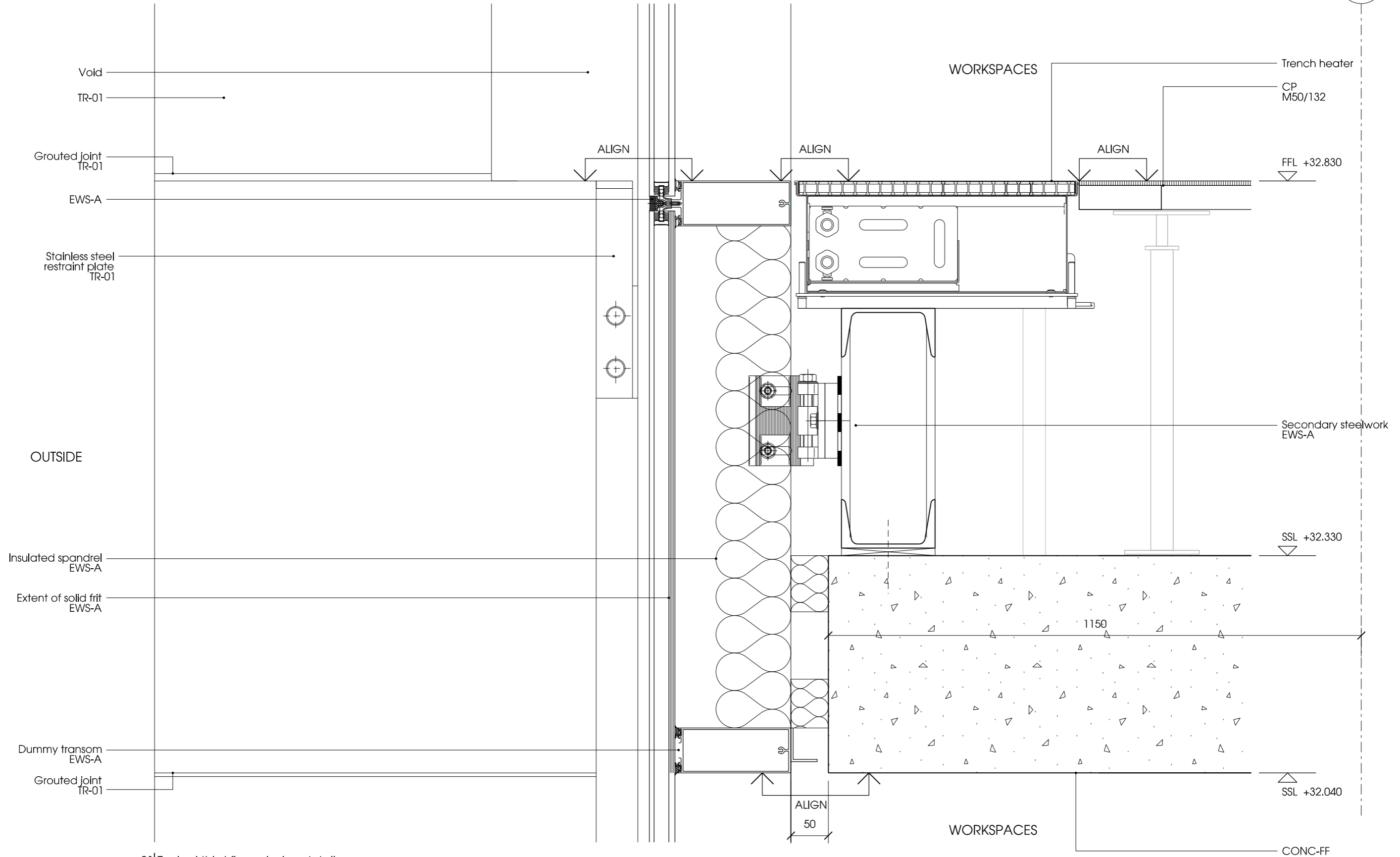
01 Typical third floor glazing detail 21_523 Refer to drawing 21_100
