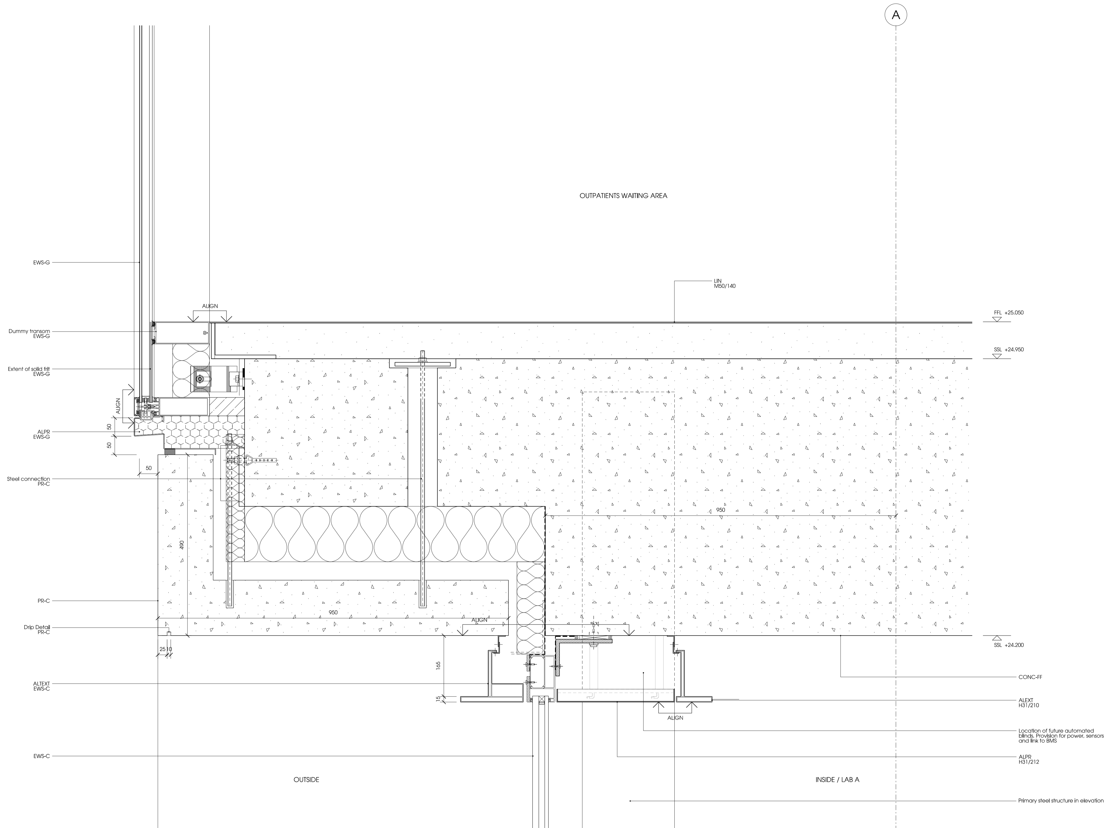
01 Typical Outpatients glazing detail to north 21_521 Refer to drawing 21_100
