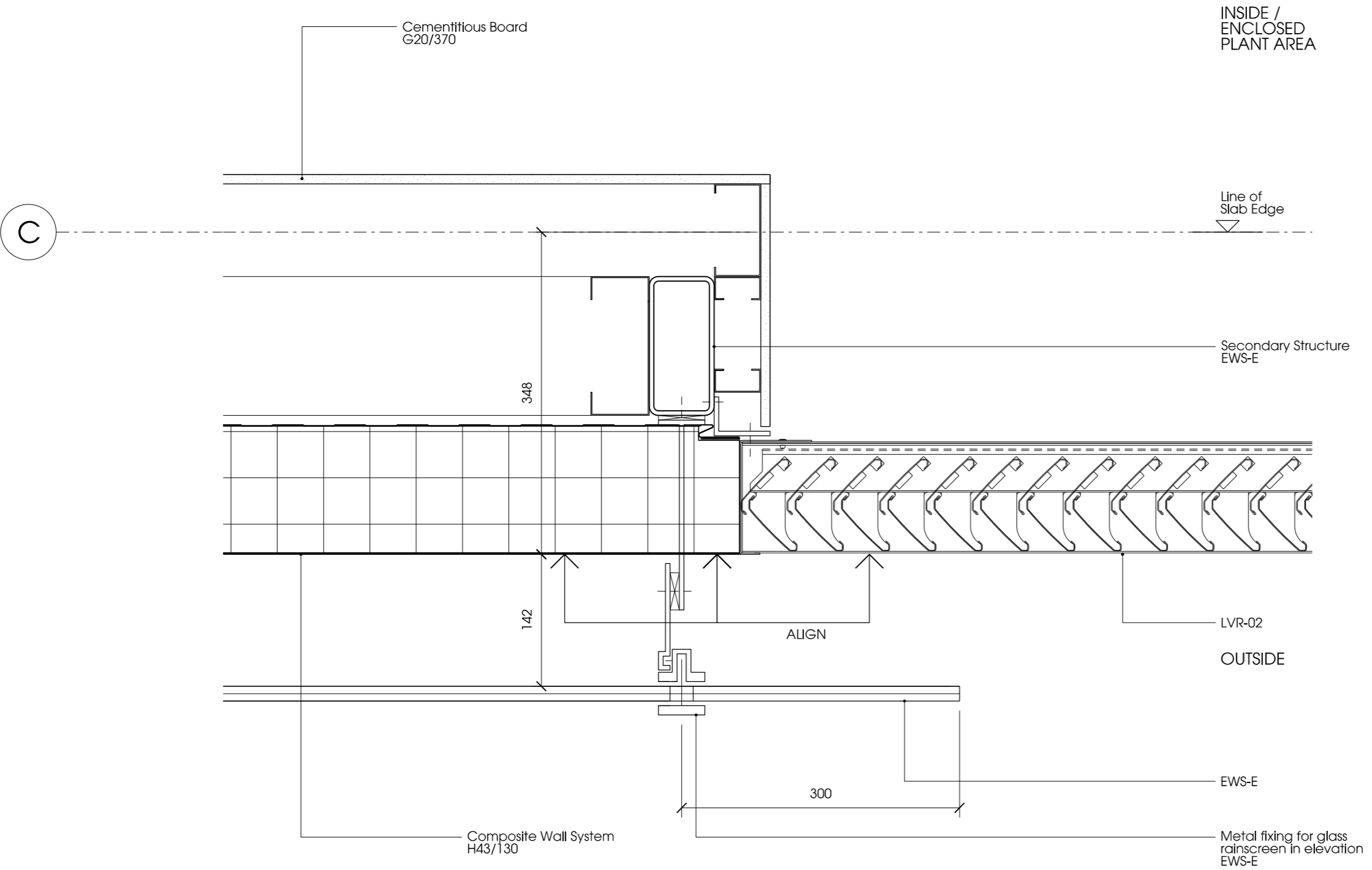
01 Typical glass rainscreen and louvre detail to south 21_454 Refer to drawing 00_331
