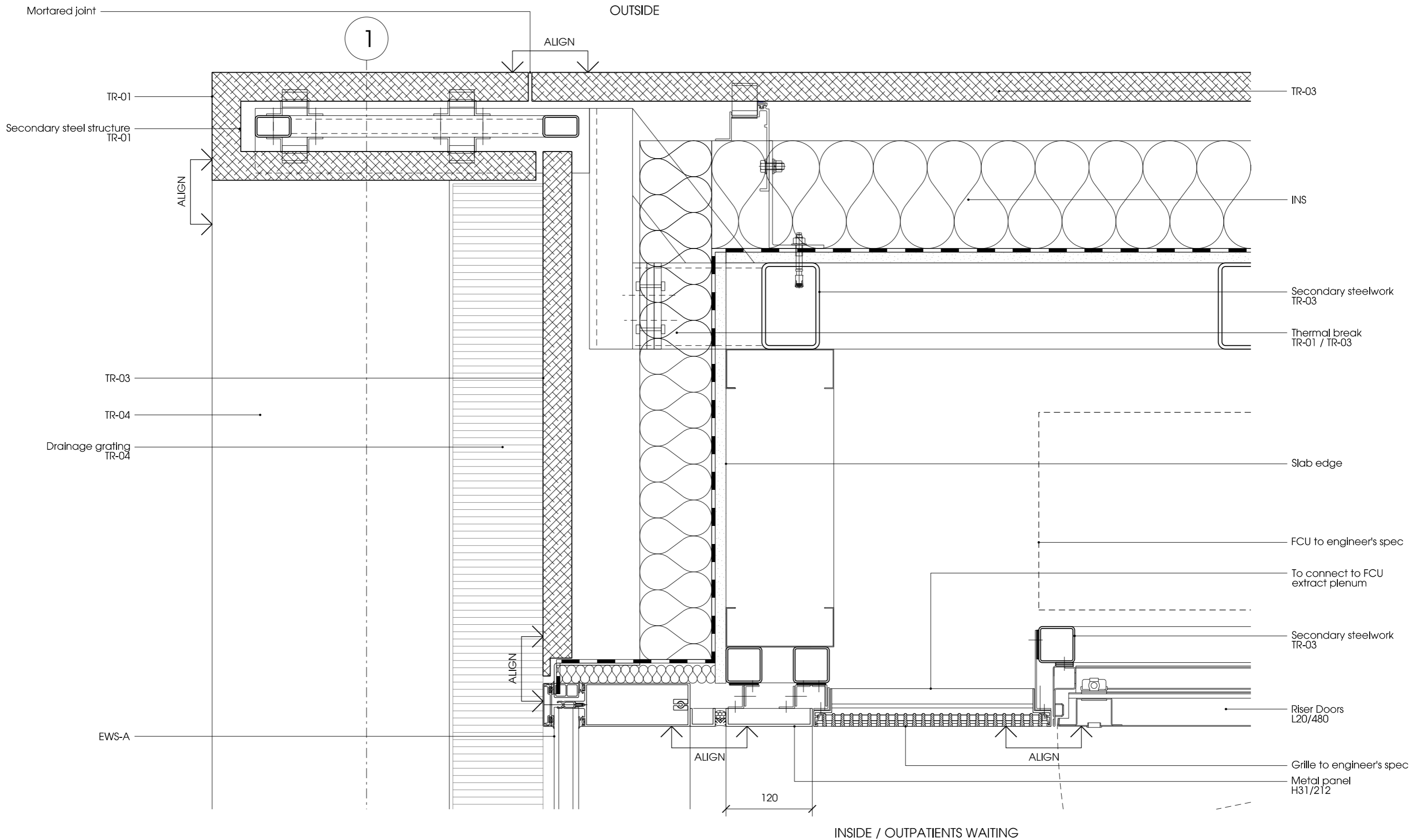
01 Terracotta fin detail north-east corner condition 21_330 Refer to drawing 00-312
