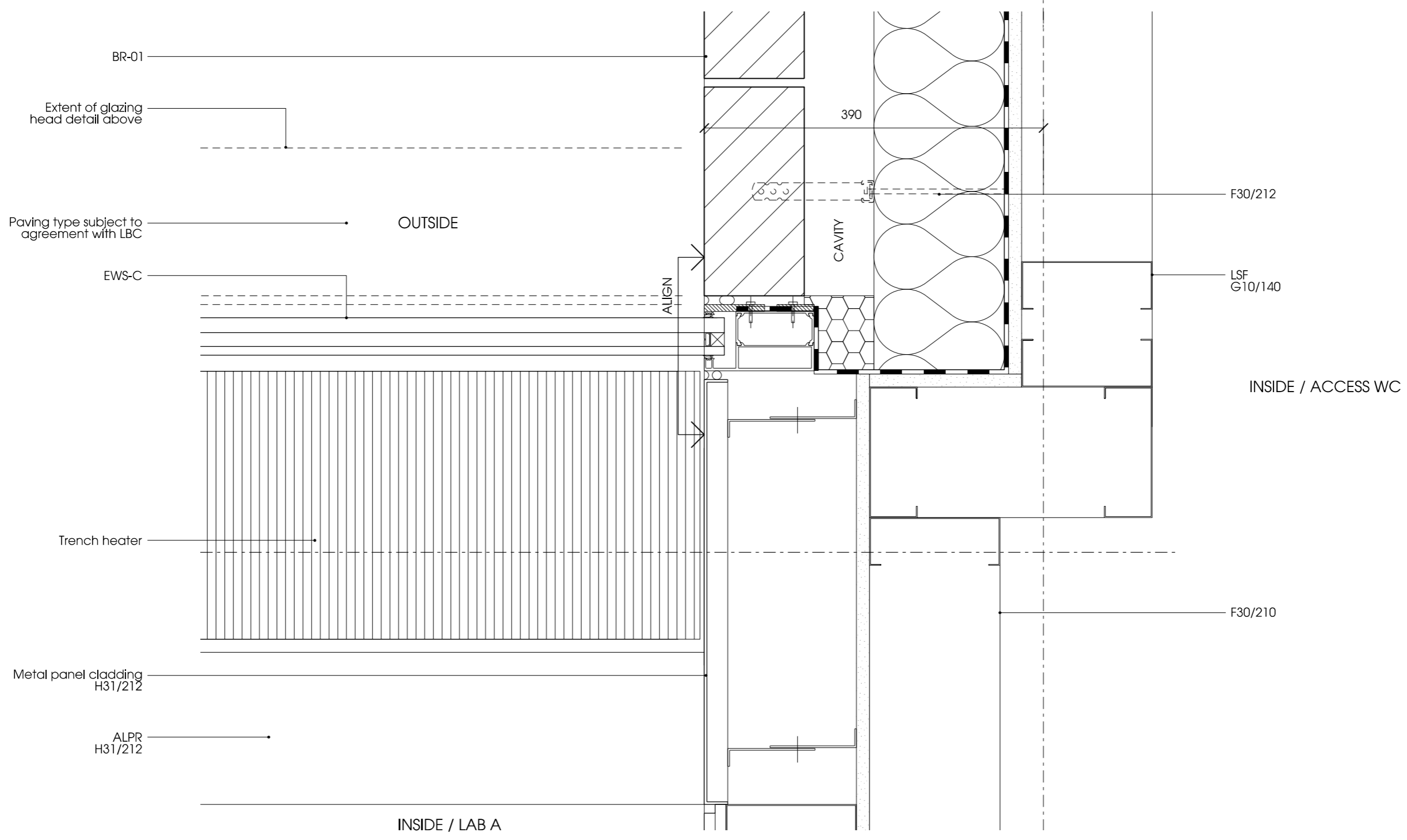
01 Lab A glazing and brickwork Interface 21_301 Refer to drawing 00_309
