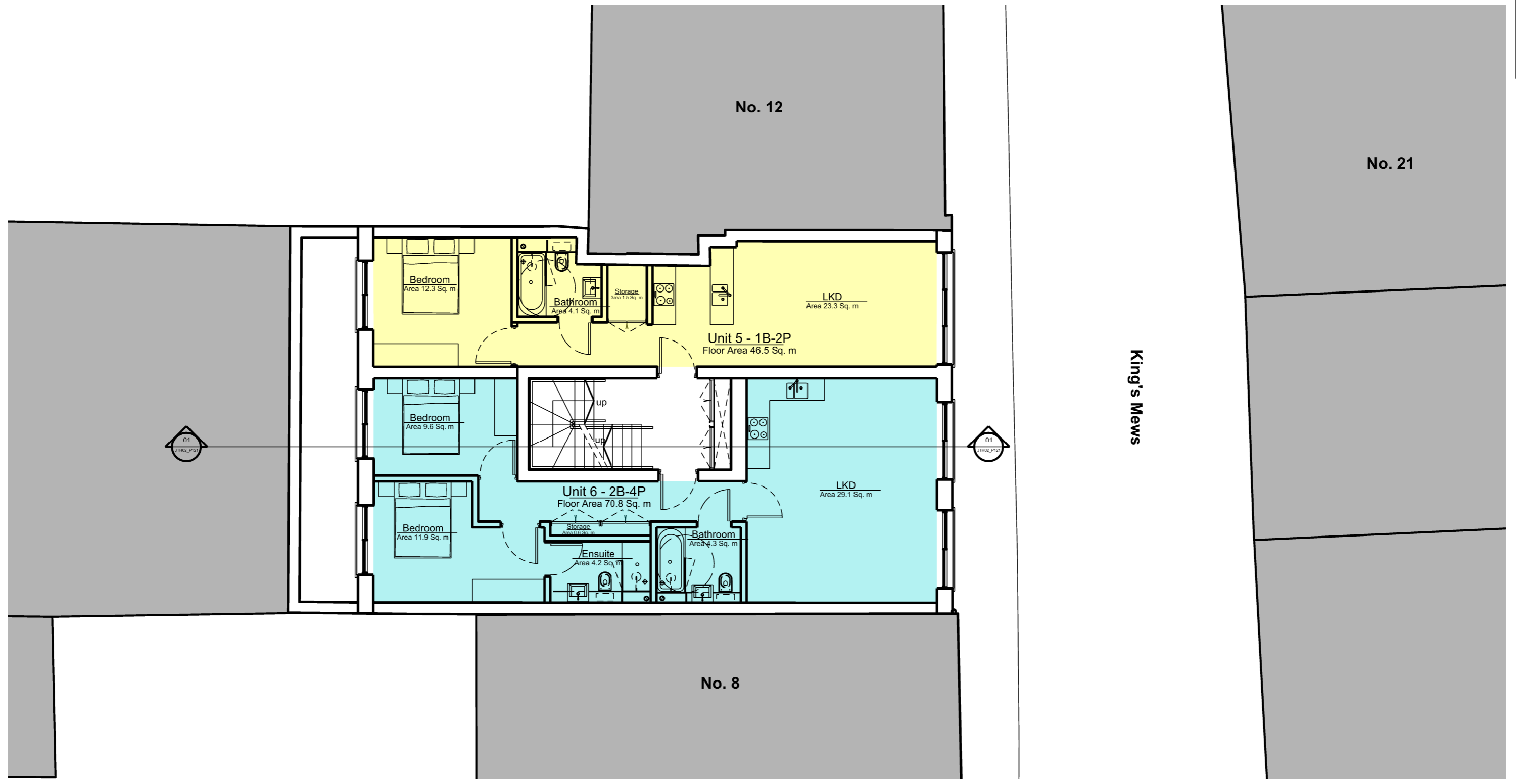
01 First Floor Plan JTH02_P101 SCALE 1:100@A3
