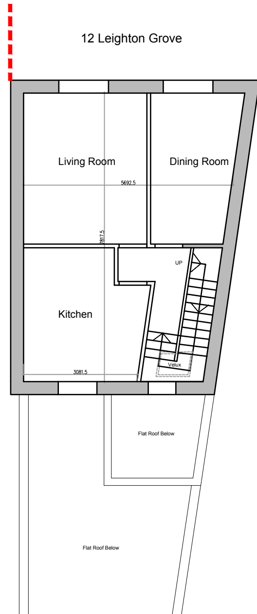
2nd Floor plan 1:100
