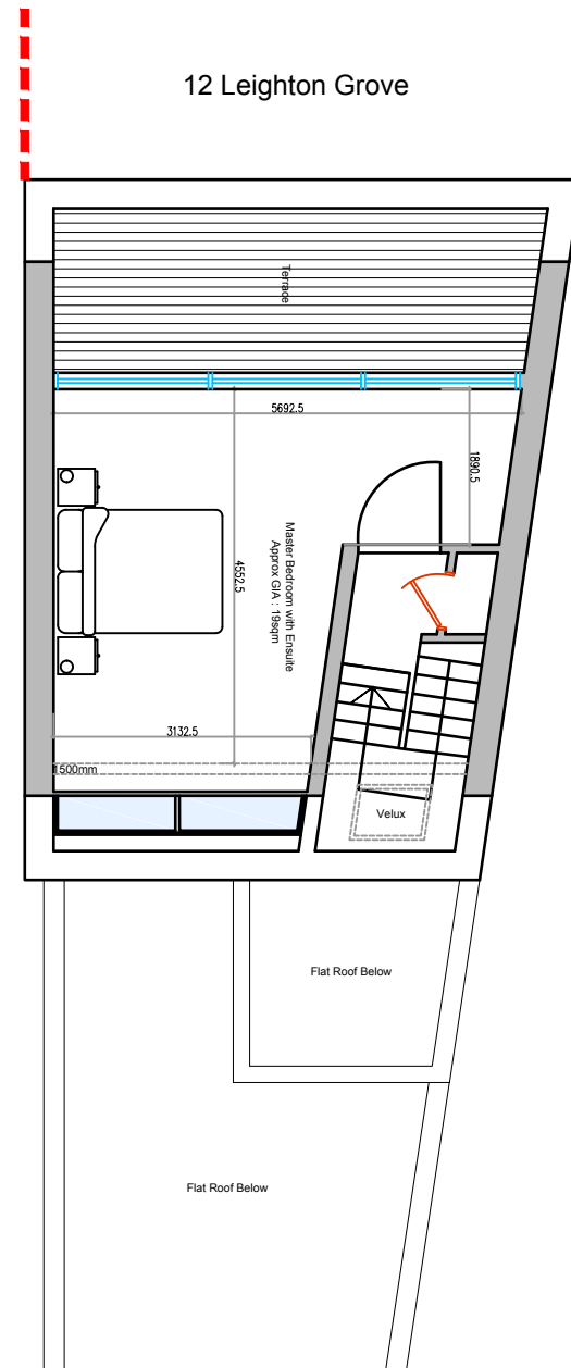
3rd Floor plan 1:100
