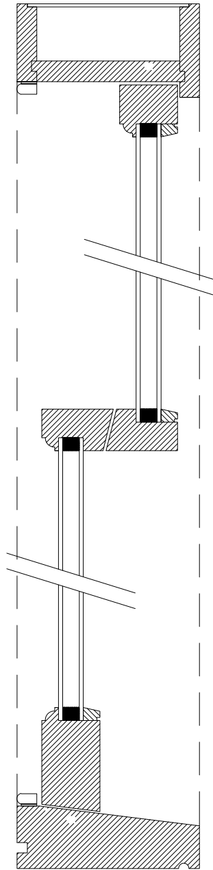
Sash Window Section (1:5)
