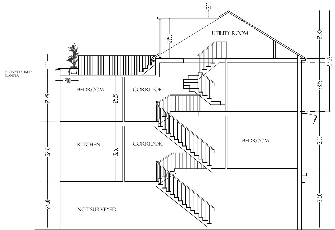
PROPOSED SECTION
