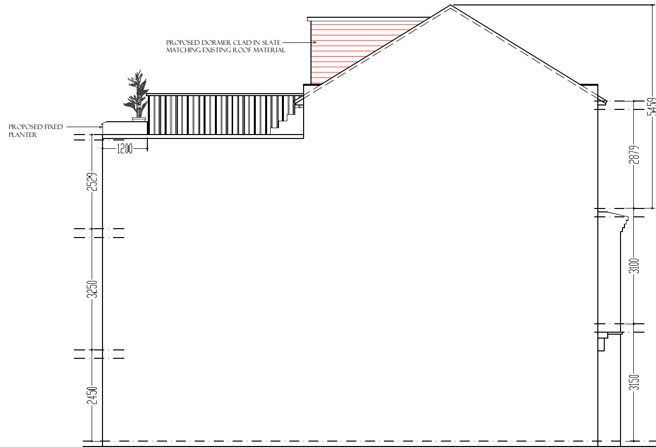
PROPOSED RIGHT SIDE ELEVATION
