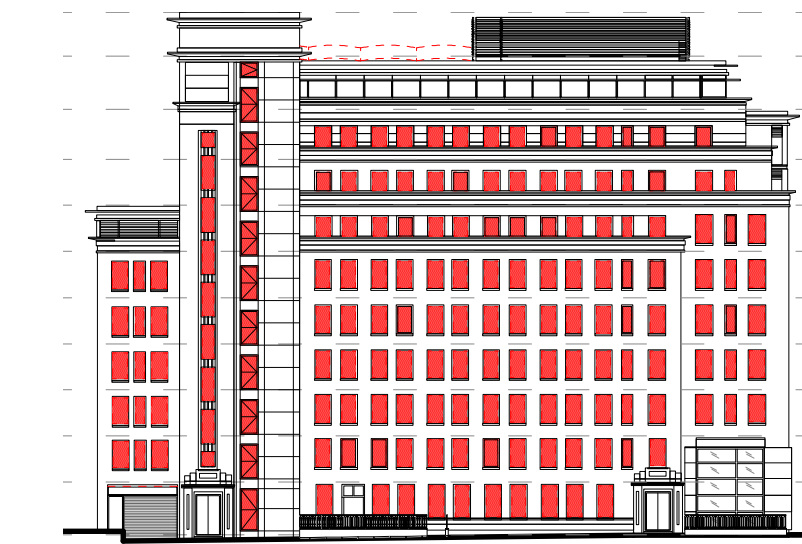
Existing East Elevation Not to scale
