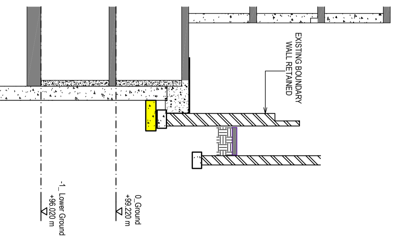
SECTION 2-2 1:100
